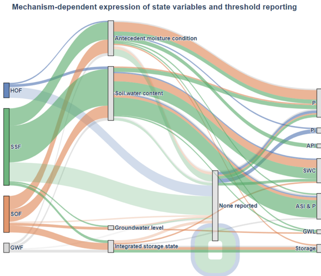
Figure 3. Sankey diagram summarizing reported indicators used to identify nonlinear runoff threshold behavior related to different dominant runoff generation mechanisms. Node height and band width are proportional to the number of reviewed catchments. The “None reported” category indicates catchments where source studies did not specify the corresponding state variable or threshold indicator. Specifically, 29 catchments did not report an explicit state variable, and 41 catchments did not report an explicit threshold indicator.
