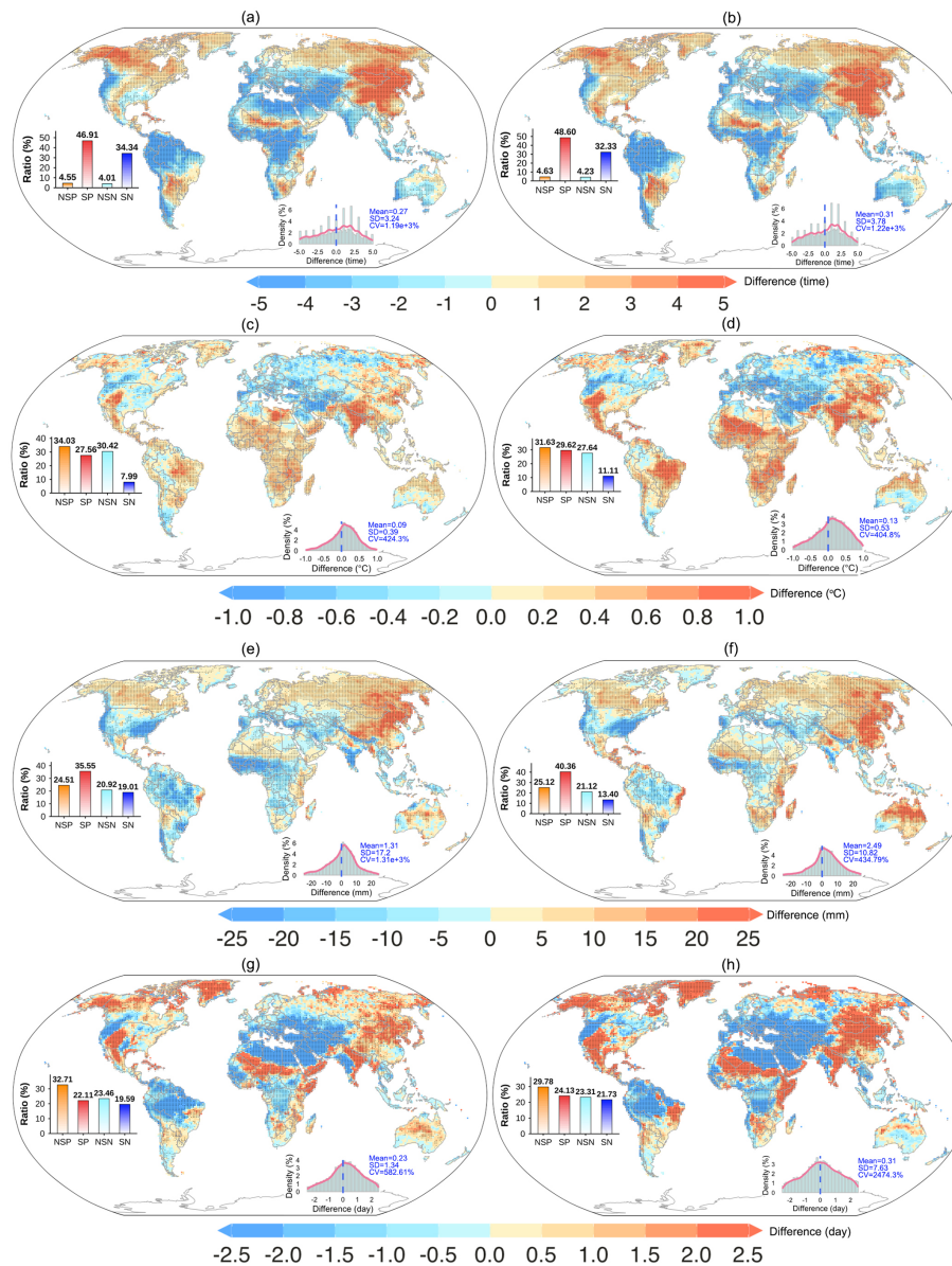
Figure 4. Spatial distribution of median differences between CHWEP and single extreme events in frequency (a, b), heatwave intensity (c, d), extreme precipitation intensity (e, f), and heatwave duration (g, h) from 2056 to 2100 under SSP2-4.5 (a, c, e, g) and SSP5-8.5 (b, d, f, h) scenarios.
