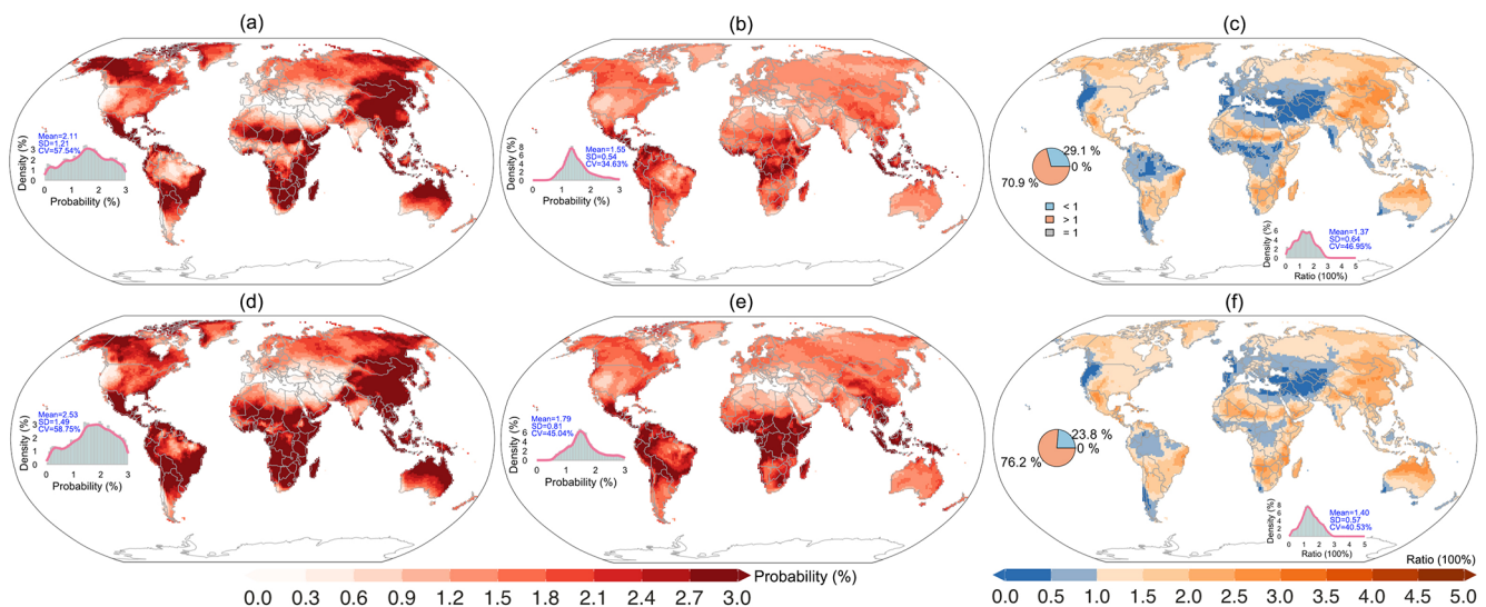
Figure 8. Spatial distributions of the mean observed probability (a, d), mean coincidence probability (b, e), and mean ratio of observed probability to coincidence probability (c, f) under the SSP2-4.5 (a–c) and SSP5-8.5 (d–f) scenarios for the period 2056–2100.
