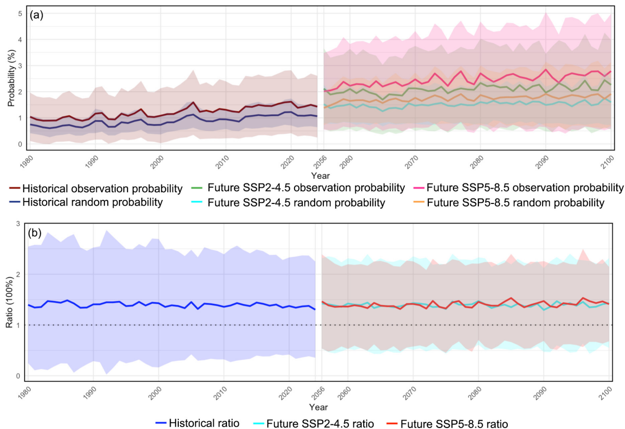
Figure 9. Changes in the observed probability and coincidence probability (a), and their ratio (b) for the global co-occurrence of heatwaves and extreme precipitation between the historical period (1980–2024) and the future period (2056–2100).
