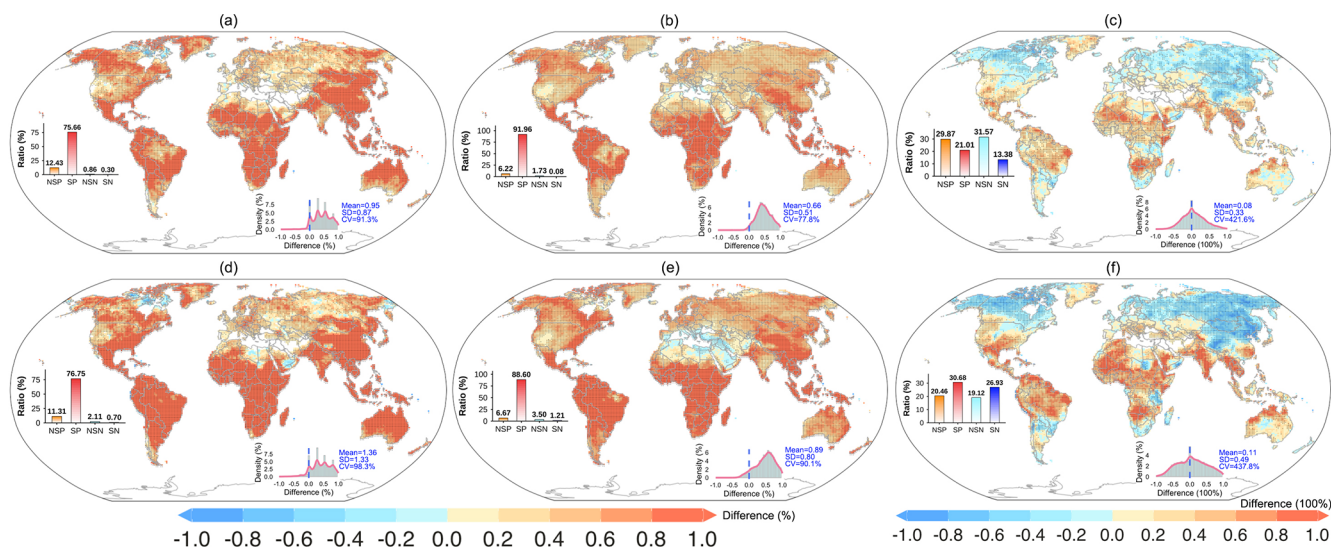
Figure 10. Spatial distribution of the differences in median values of observed probability (a, d), coincidence probability (b, e), and their ratio (c, f) for the co-occurrence of heatwaves and extreme precipitation between the future period (under SSP2-4.5 a–c and SSP5-8.5 d–f scenarios) and the historical period.
