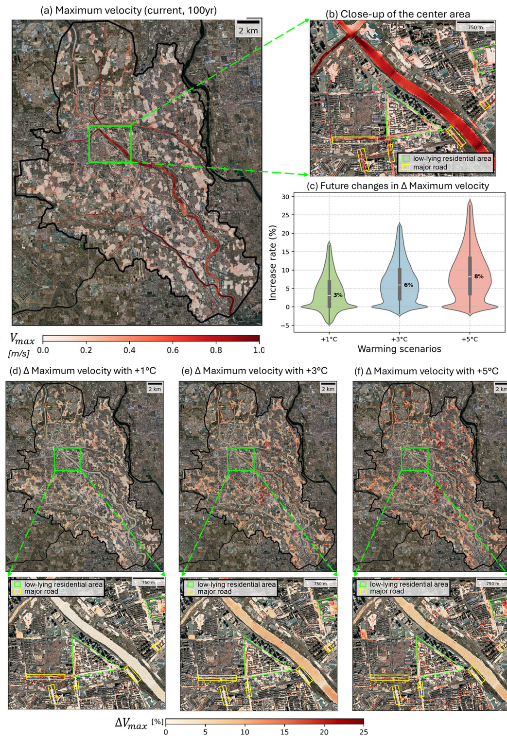
Figure 9. (a) The maximum velocity for 100-year rainfall return level under the current climate, (b) zoom-in to the BMC center, (c) future changes of maximum velocity under different regional future warming levels, and its spatial distribution of those changes within BMC region under 1 (d), 3 (e), 5 °C (f) warming level. Basemaps are derived from ESRI World Imagery (Credit: Esri, TomTom, Garmin, FAO, NOAA, USGS, © OpenStreetMap contributors, and the GIS User Community).
