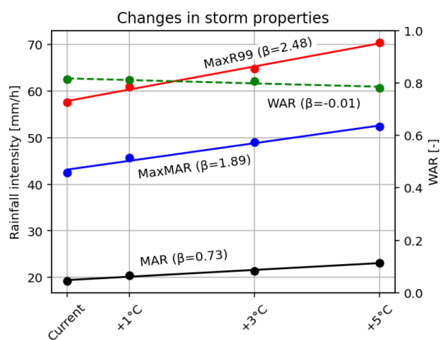
Figure 11. Future changes in mean areal rainfall (MAR, black line), maximum mean areal rainfall (MaxMAR, blue line), 99th percentile of extreme rainfall at the grid-scale (MaxR99, red line), and area of the storm (WAR, green dash) for the 100-year storms in BMC.
