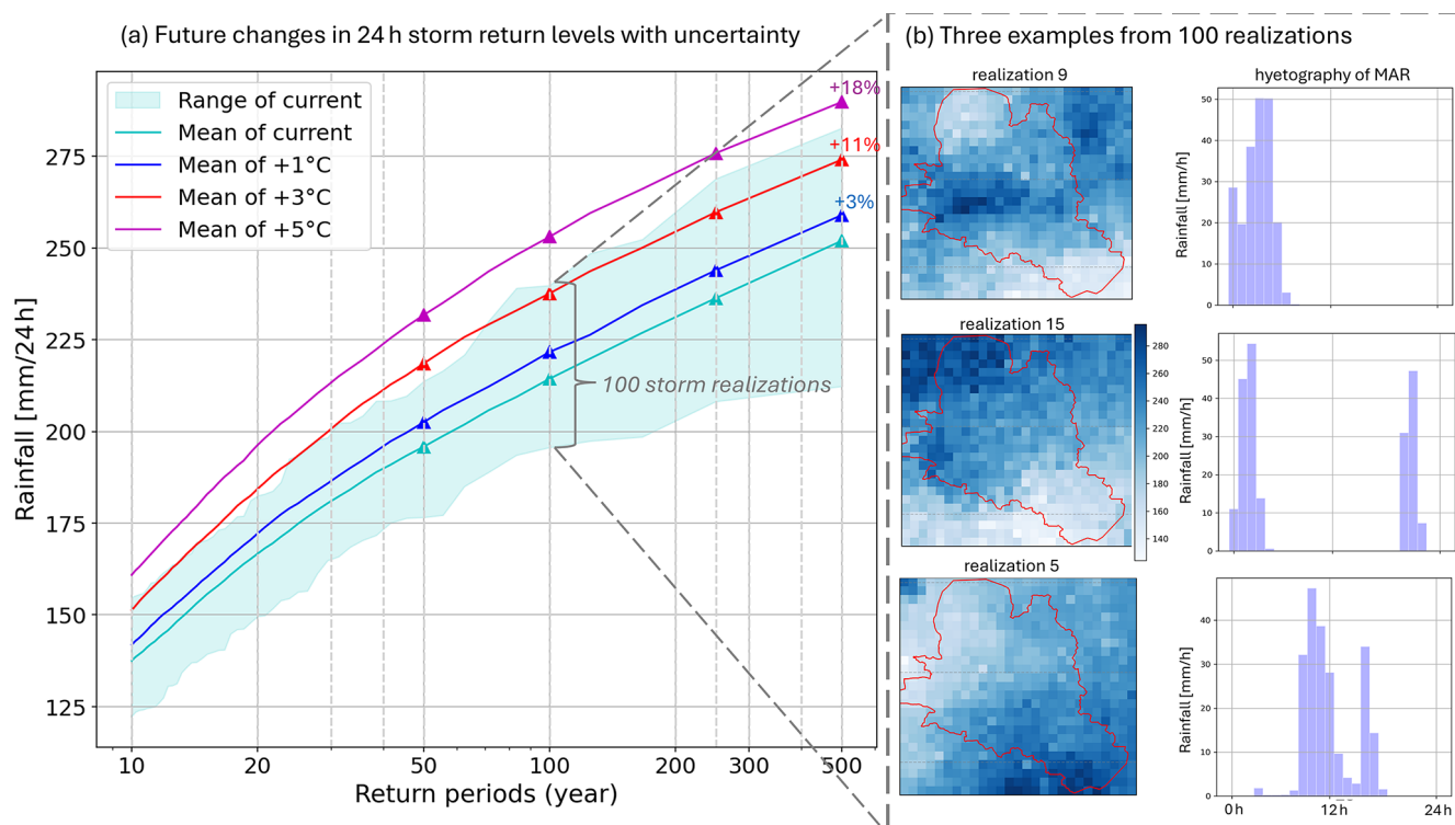
Figure 6. (a) Return levels of averaged rainfall over the BMC for 24 h storm event and their natural variability computed from 100 realizations of storm events, (b) examples of three 24 h storm realizations, illustrating their spatial (left column) and temporal (right column) distributions.
