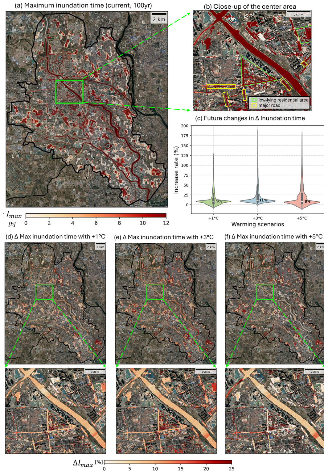
Figure 8. (a) The inundation duration for 100-year rainfall return level under the current climate, (b) zoom-in part in the BMC centre, (c) future changes of inundation duration under different regional warming levels, and its spatial distribution of those changes within BMC region under 1 (d), 3 (e), 5 °C (f) warming levels. Basemaps are derived from ESRI World Imagery (Credit: Esri, TomTom, Garmin, FAO, NOAA, USGS, © OpenStreetMap contributors, and the GIS User Community).
