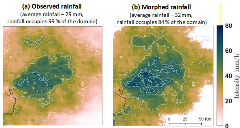
Figure 2. (a) An example of an observed rainfall field (1 h and 1 km resolution). (b) Future projected rainfall field for a 7\% \text{ }^{\circ}\text{C}^{-1} increase in mean areal rainfall intensity and 8\% \text{ }^{\circ}\text{C}^{-1} decrease in rainfall-affected area under 2^{\circ}\text{C} regional warming.
