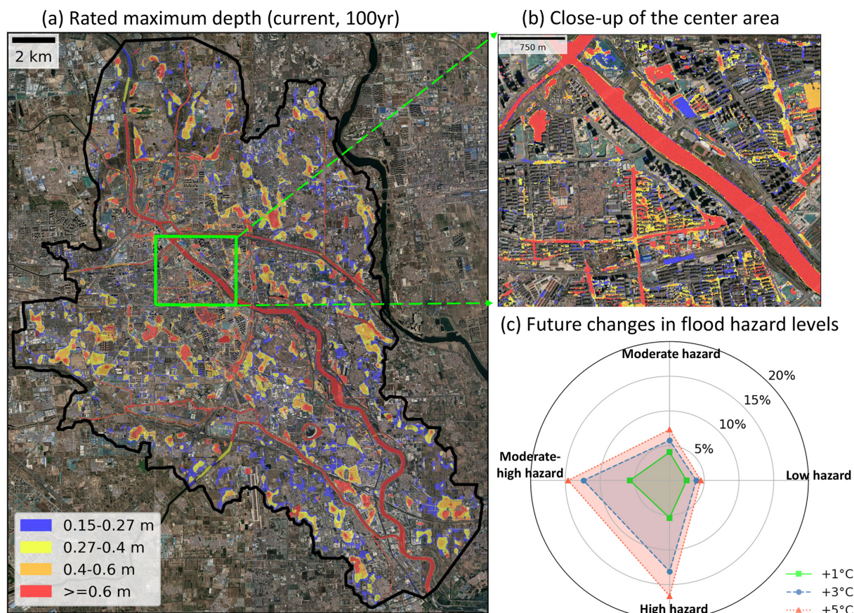
Figure 10. (a) Flood hazard for 100-year rainfall return level under the current climate, (b) close-up of the BMC centre, and (c) changes in flood hazards assessments within BMC under different regional warming levels. Basemaps are derived from ESRI World Imagery (Credit: Esri, TomTom, Garmin, FAO, NOAA, USGS, © OpenStreetMap contributors, and the GIS User Community).
