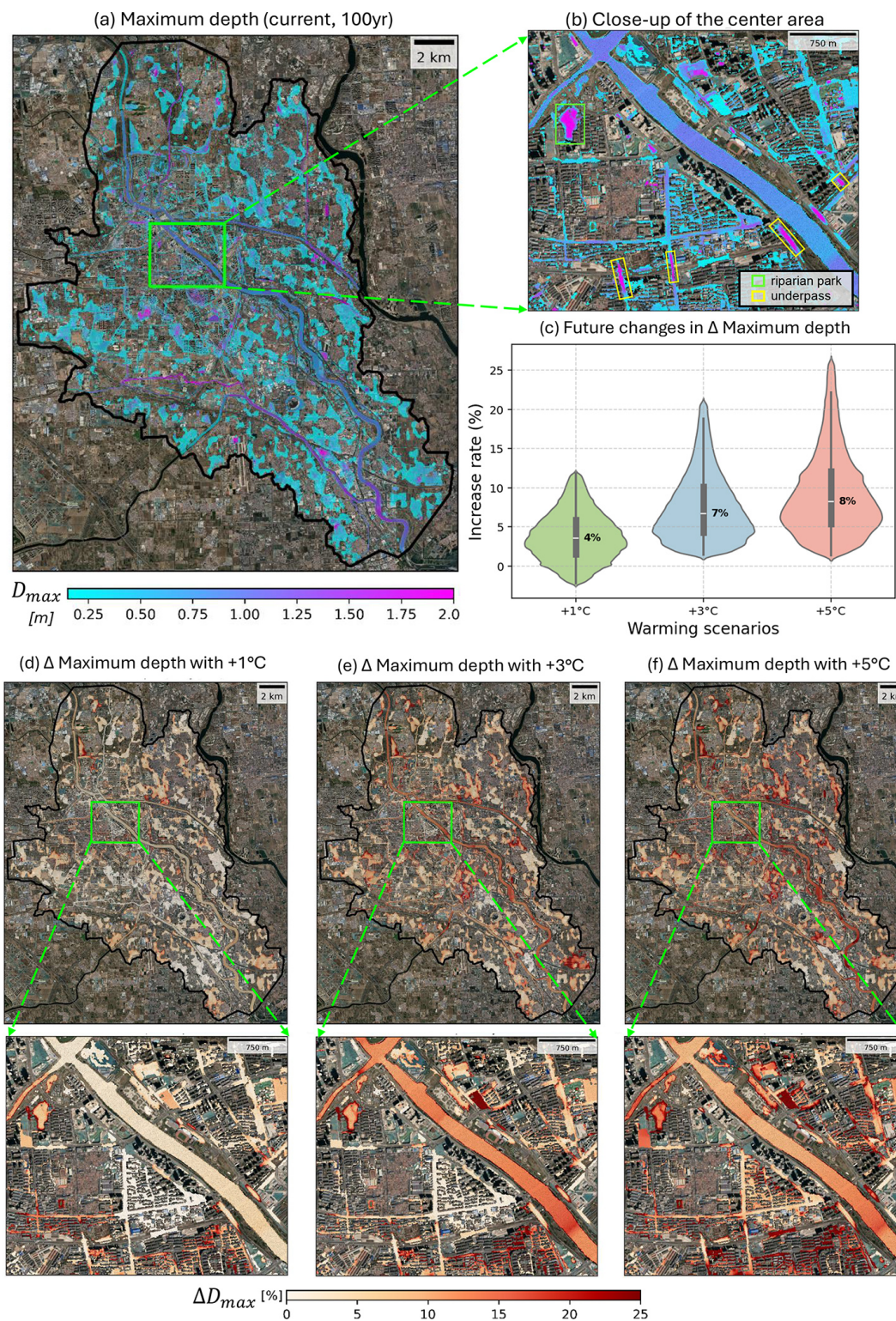
Figure 7. (a) The maximum flood depth for 100-year rainfall return level under the current climate, (b) zoom-in part in the BMC centre, (c) future changes of maximum flood depth under different regional warming levels, and its spatial distribution of those changes within BMC region under 1 (d), 3 (e), 5 °C (f) warming levels. Basemaps are derived from ESRI World Imagery (Credit: Esri, TomTom, Garmin, FAO, NOAA, USGS, © OpenStreetMap contributors, and the GIS User Community).
