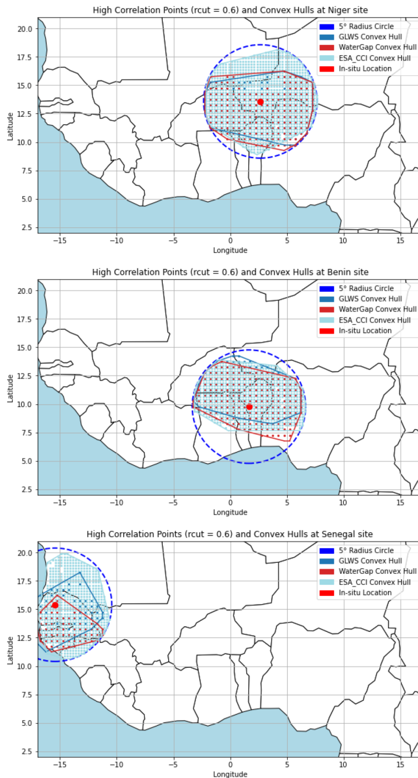
Figure 6. Spatial footprint of SM products represented by a blue circle with a radius of 5° around each site, indicated in red. The convex hulls in light and dark blue represent the areas for which ESA CCI and GLWS2.0 exceed the specified cutoff threshold of 0.6, respectively. Figure created by the authors using datasets described in the manuscript. ESA CCI data courtesy of ESA. GLWS2.0 data courtesy of the GLWS team. WaterGAP data courtesy of the WaterGAP project. CLM5 data courtesy of NCAR/UCAR.
