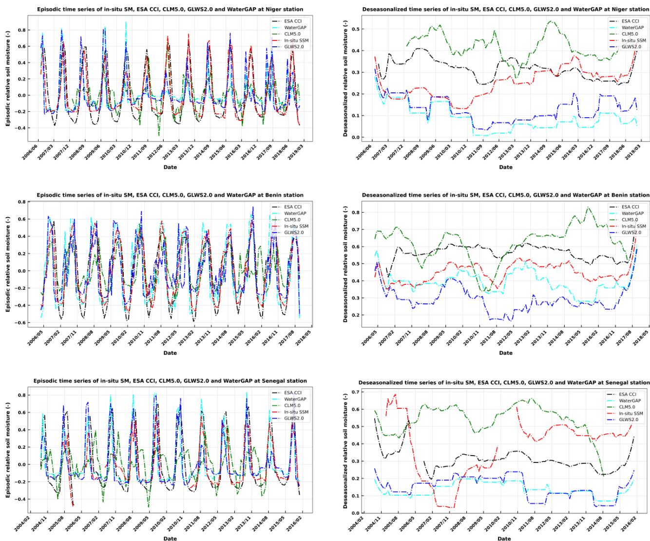
Figure 4. Episodic and deseasonalized SM time series for the three study sites (Niger, Benin, and Senegal).
