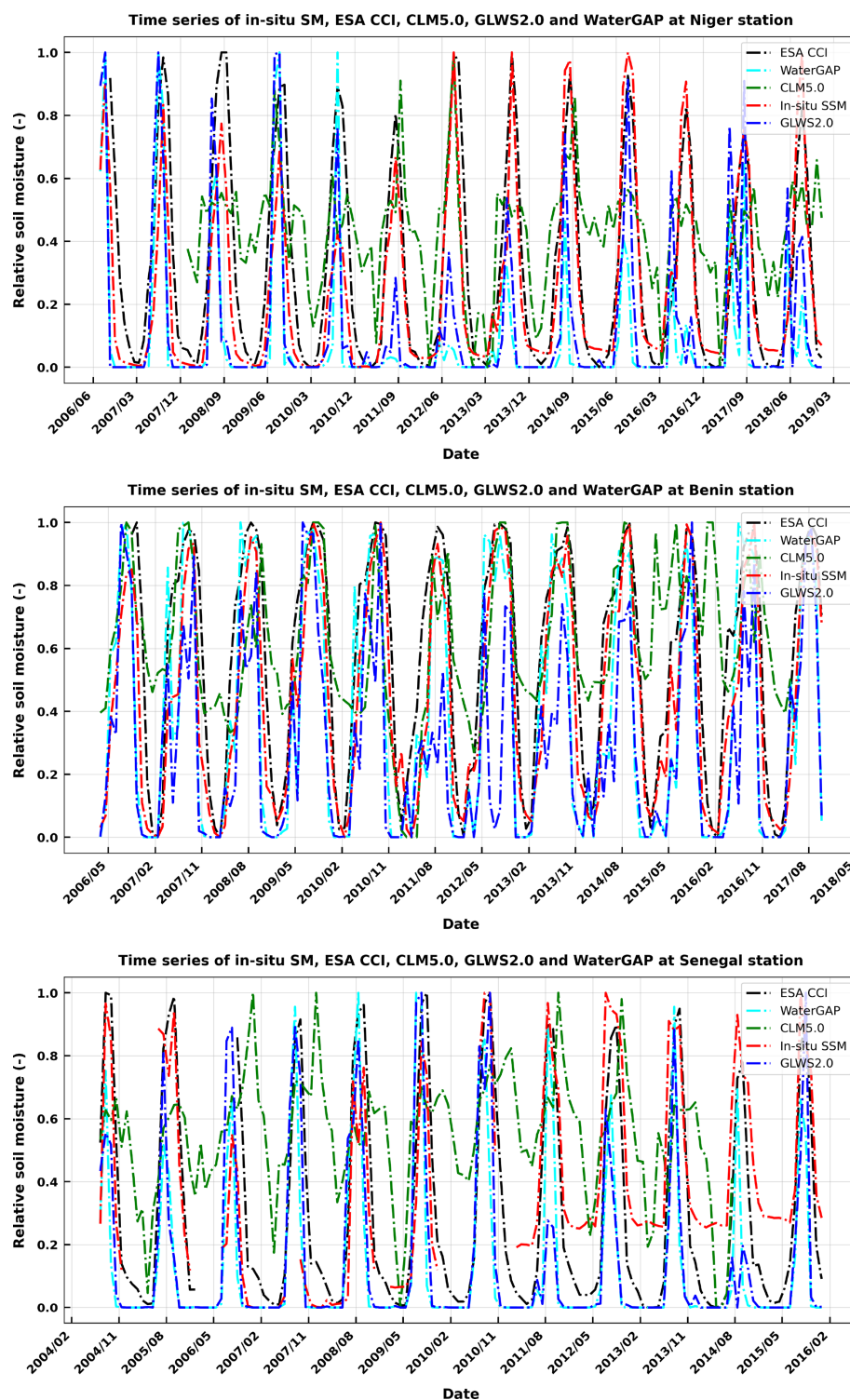
Figure 3. Normalized SM time series for in situ measurements, ESA CCI, GLWS2.0, WaterGAP, and CLM5.0 at three distinct study sites at a depth of 5 cm.
