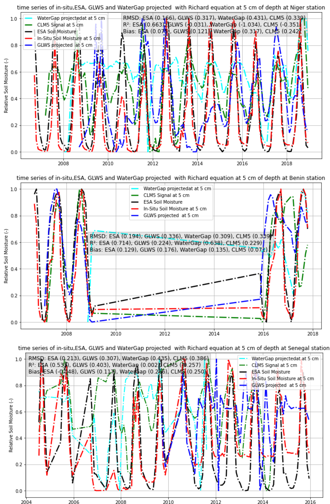
Figure 7. SM time series for in situ measurements, ESA CCI, GLWS2.0, WaterGAP, and CLM5.0 at three distinct study sites, projected at a depth of 5 cm. ESA CCI data courtesy of ESA. GLWS2.0 data courtesy of the GLWS team. WaterGAP data courtesy of the WaterGAP project.
