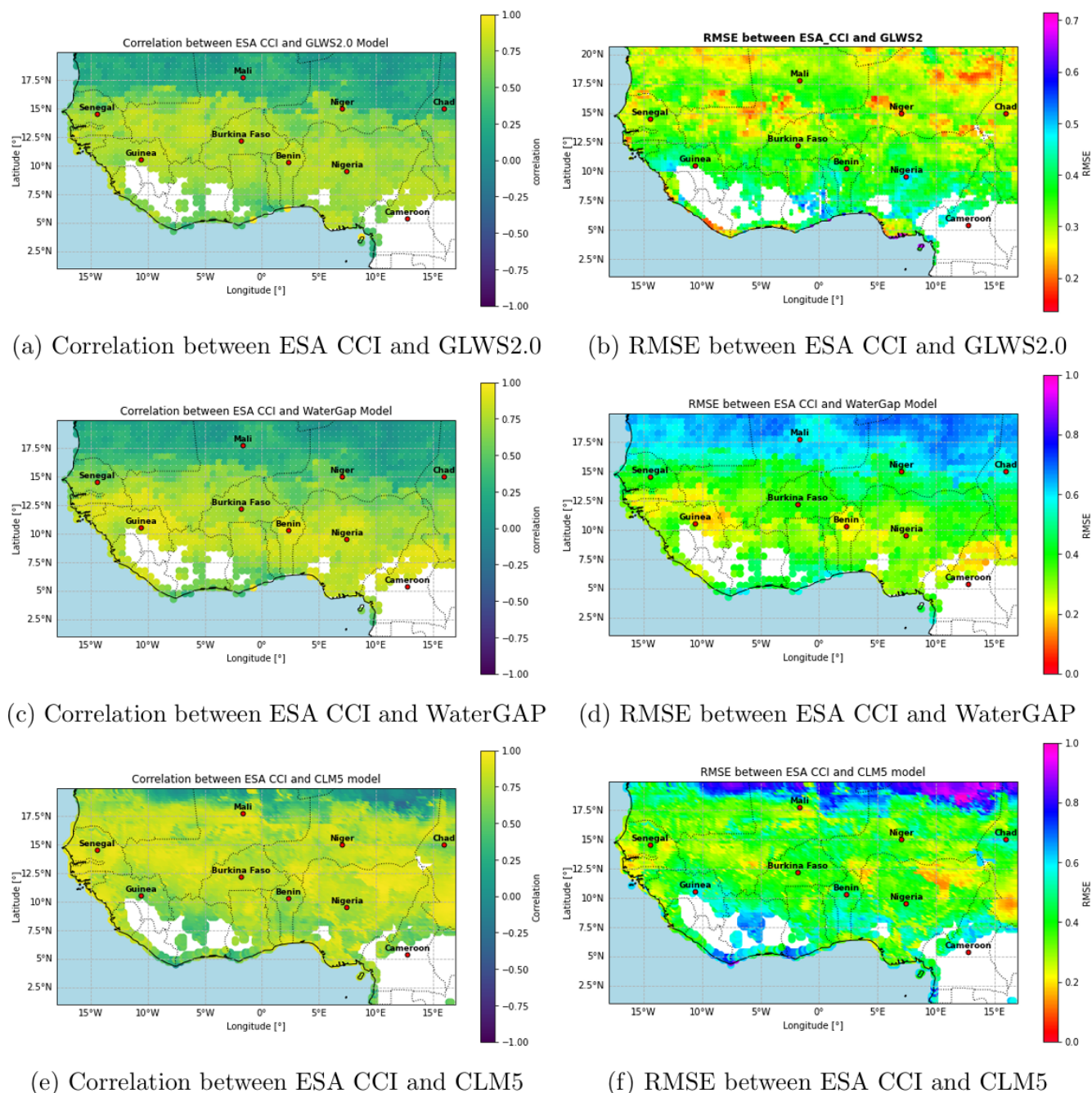
Figure 5. Pearson correlation coefficient ( R ) and RMSE metrics illustrating the performance of GLWS2.0, WaterGAP, and CLM5 models relative to the ESA CCI grid. Figure created by the authors using datasets described in the manuscript.
