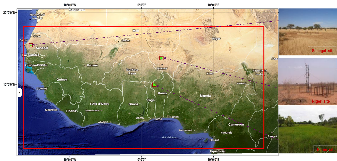
Figure 1. Location of the three meso-scale study sites in West Africa where in situ SM stations from the ISMN are installed: Benin, Niger, and Senegal. Green dots indicate the locations of the individual SM stations (four in Benin, three in Niger, and one in Senegal). Red squares represent the 0.25^\circ satellite grid cells used to compare satellite and model SM products with the in situ observations. The red rectangle delineates the regional domain used for the gridded validation between ESA CCI SM and the land surface models (CLM5.0, GLWS2.0, and WaterGAP). Figure is created by the authors. ISMN data courtesy of ISMN. ESA CCI SM data courtesy of ESA. CLM5.0 data courtesy of NCAR/UCAR. GLWS2.0 data courtesy of the GLWS team. WaterGAP data courtesy of the WaterGAP project. Photos used are adapted from Louvet et al. (2015).
