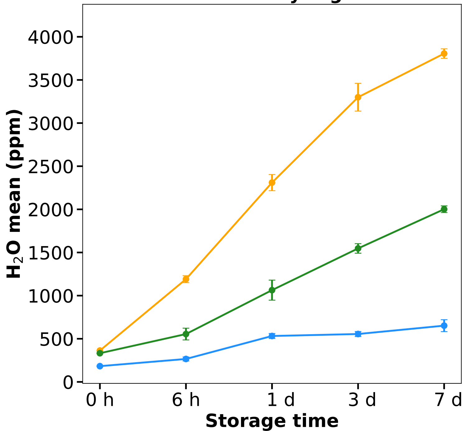
0.80 mm syringe
