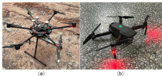
Figure 1. Field deployment of the UAV sensing system, including the (a) DJI Matrice 600 platform carrying the PoLRa v3.1 dual-polarized L-band radiometer and the (b) DJI Mavic 2 Enterprise Advanced used for RGB-TIR survey.
