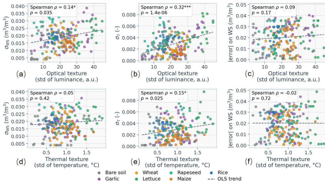
Figure 7. Relationships between footprint-scale optical and thermal texture and retrieval uncertainty. Panels (a)–(c) show optical texture versus posterior soil-moisture standard deviation, posterior \tau uncertainty, and absolute soil-moisture error. Panels (d)–(f) show the corresponding thermal-texture relationships.
