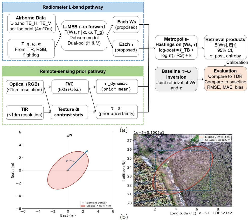
Figure 3. Workflow of the Bayesian joint retrieval. The workflow includes data preprocessing, radiometric brightness-temperature quality control, footprint-consistent RGB-TIR aggregation, Bayesian retrieval with RGB-TIR-informed priors, TDR validation labels, baseline comparison, and uncertainty evaluation. Panel (b) illustrates the nominal 4 \times 7 m heading-oriented ellipse used as a geometry-informed approximation of microwave support when summarizing high-resolution optical and thermal information before Bayesian inversion.
