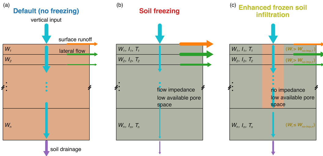
Figure 1. Conceptual scheme of the soil water balance in SVS (evapotranspiration is not shown here) for (a) the default configuration without soil freezing, (b) the soil freezing configuration and (c) the configuration of enhanced frozen ground infiltration. W denotes the water content of layer i while I and T denote the ice fraction and the temperature of layer i , respectively, on (b) and (c). Vertical downward water flux through the soil column is shown by blue arrows while orange, green and purple arrows correspond to surface runoff, lateral flow and soil drainage, respectively. The relative size of the arrows represents the relative magnitude of the fluxes in each configuration.
