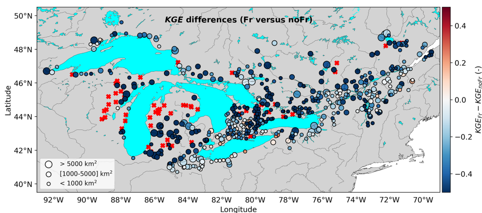
Figure 3. Map of the KGE differences between the soil freezing (Fr) experiment and the experiment without soil freezing (noFr) over the Great-Lakes and Saint-Lawrence domain for the 2016–2021 period. Degradations of the KGE with the Fr experiment (negative KGE differences) are represented by cold-colored dots. Red crosses show stations excluded from the comparison (see Sect. 2.4.1).
