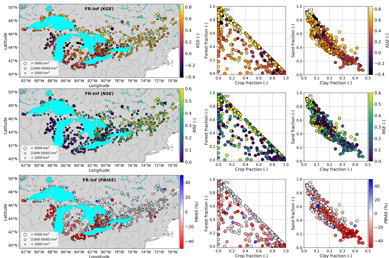
Figure 7. Spatial performance and catchment characteristics for the Fr-Inf experiment (2016–2021). Left panels (a), (d), (g) show the Great Lakes and Saint-Lawrence domain with KGE, NSE, and PBIAS at each station. Right panels (b), (c), (e), (f), (h), (i) show corresponding forest-crop and sand-clay fractions categorized by performance scores. In (a) to (f), a good performance of the model is represented by yellow shades. In (g) to (i), underestimation of streamflow is shown by red colors while an overestimation is shown by blue colors with pale red and blue dots show a low absolute bias.
