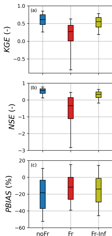
Figure 6. Boxplots of streamflow performances for the KGE in (a), the NSE in (b) and the PBIAS in (c) for the three configurations (noFr, Fr, Fr-Inf) in the Great-Lakes and Saint-Lawrence domain for the 2016–2021 evaluation period. Details on boxplot representation are given in the legend of Fig. 4. The target value for the KGE and NSE is 1.0 while the target value for the PBIAS is 0.0.
