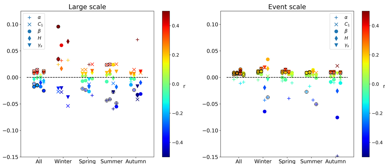
Figure 9. Slope (°C -1 ) of the linear regression of the value of the studied parameters vs. \langle T \rangle at both large and event scales for each measurement campaign for all events (left, it corresponds to values displayed in Tables 3 and 5) as well as per season. For each season, the 4 “columns” correspond in that order to all campaigns together, ENPC Campus, SIRTa and Pays d’Othe. Symbols are colored according to Pearson coefficient of correlation. The ones circled correspond to cases for which the null hypothesis of no trend was rejected.
