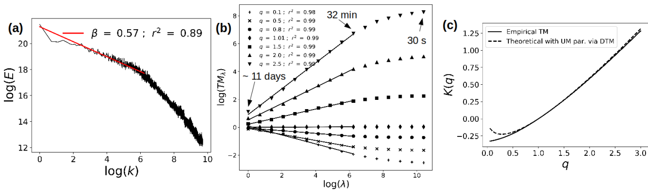
Figure 4. For the campaign “ENPC campus” with ensemble analysis for large scales. (a) Spectral analysis, i.e. Eq. (5) in log-log. (b) TM analysis, i.e. Eq. (1) in log-log. (c) Scaling moment function K(q) : empirical estimate and theoretically fitted shape using UM parameters from DTM analysis.
