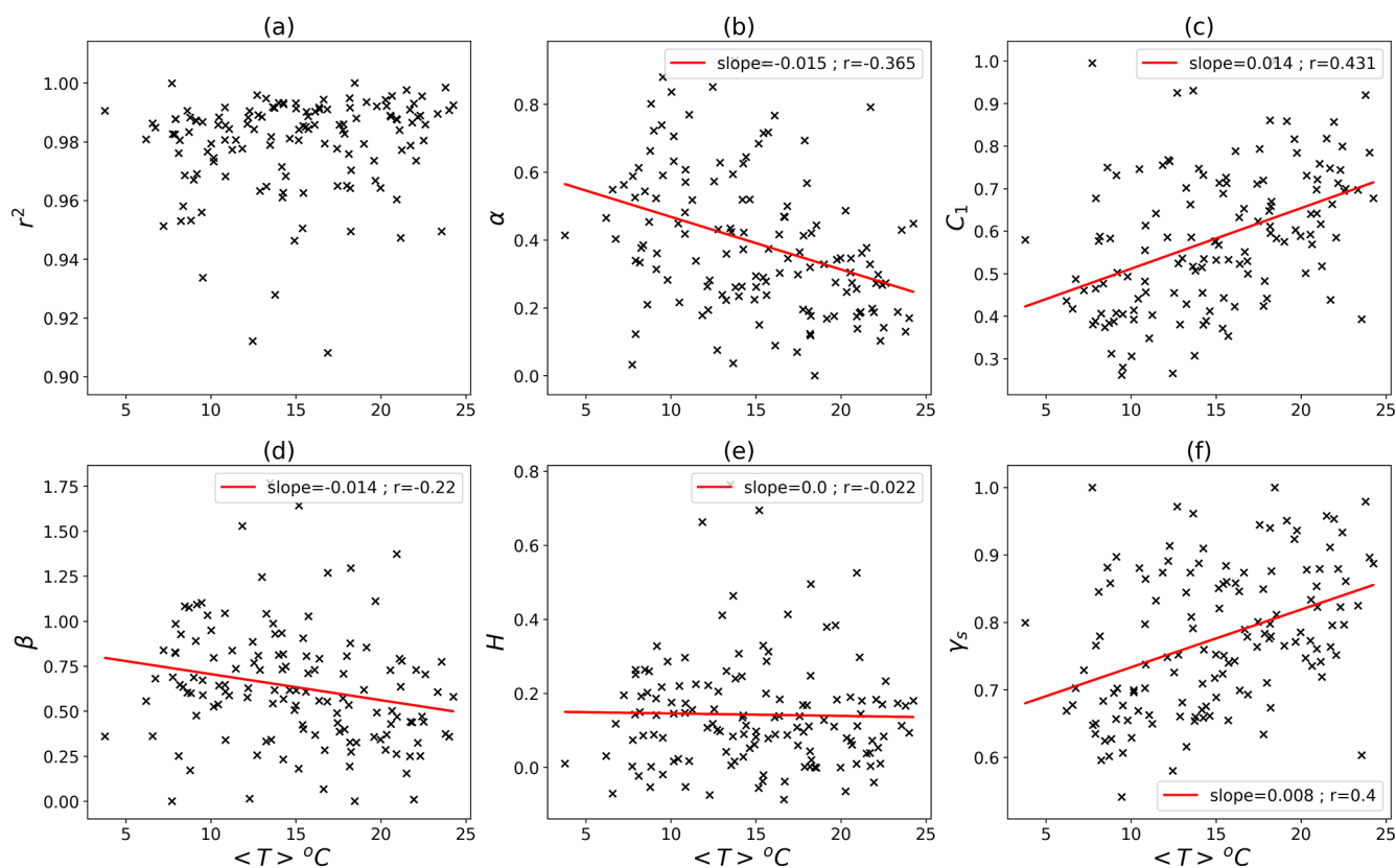
Figure 5. For the campaign “ENPC campus” with individual sample analysis for large scales: r^2 for q = 1.5 in TM analysis (a), \alpha (b), C_1 (c), \beta (d), H (e) and \gamma_s (f) vs. \langle T \rangle
