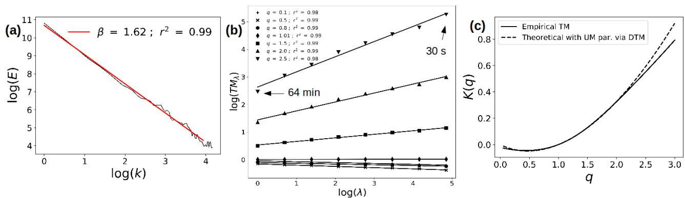
Figure 7. For the campaign “ENPC campus” with ensemble analysis at event scale. (a) Spectral analysis, i.e. Eq. (5) in log-log. (b) TM analysis, i.e. Eq. (1) in log-log. (c) Scaling moment function K(q) : empirical estimate and theoretically fitted shape using UM parameters from DTM analysis.
