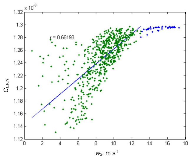
Figure 7. Dependence of the 10 m neutral transfer coefficient for moisture ( C_{E10N} ) on the 2 m wind speed ( w_2 ) on the basis of 30 min mean values observed over Lake Zub/Priyadarshini (2017–2018).
