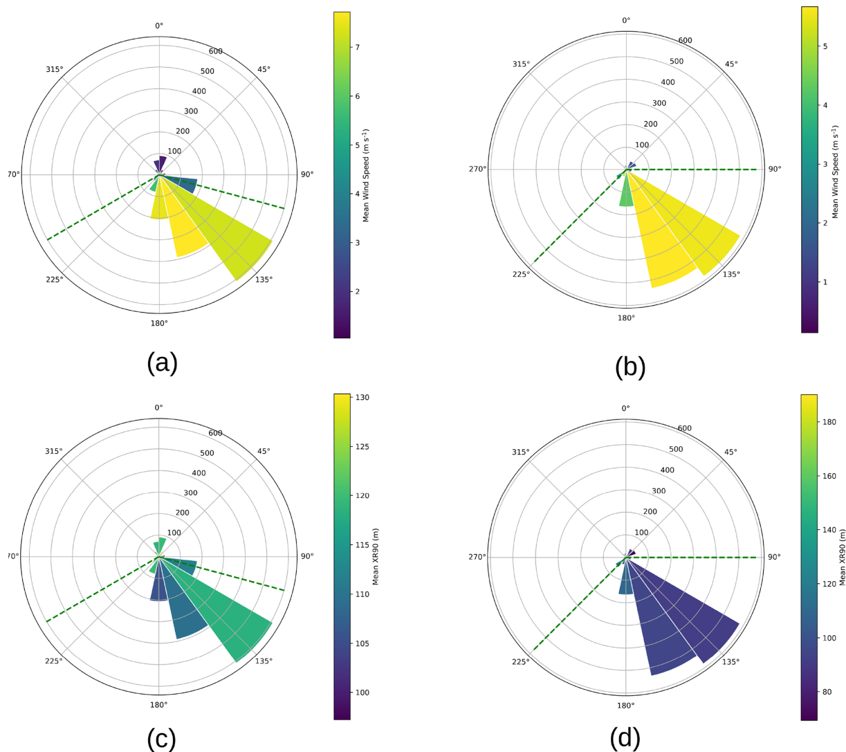
Figure 5. The wind speed and direction measured at IRGASON site ( a : Lake Zub/Priyadarshini, and b : Lake Glubokoe) and the footprint length estimate ( XR_{90} , m) ( c : Lake Zub/Priyadarshini, and d : Lake Glubokoe). The green lines indicate the footprint sector.
