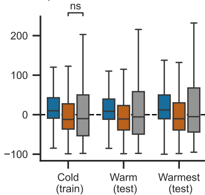
b) Low flow bias
