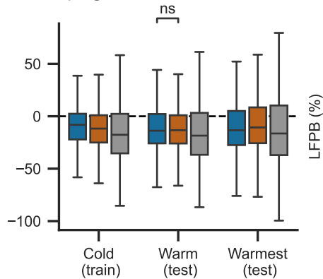
a) High flow bias
