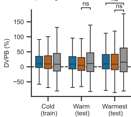
c) Drought volume bias
