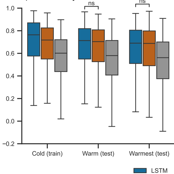
a) Model accuracy
