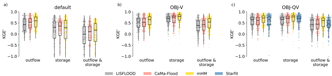
Figure 6. Comparison of the model performance depending on the reservoir routine. The panels correspond to three of the experiments: (a) default parameters, (b) calibration of storage (OBJ-V), (c) bivariate calibration of outflow and storage (OBJ-QV). Within each panel, three groups of box plots show the performance in terms of outflow, storage, and both variables together. Four reservoir routines are compared – LISFLOOD, CaMa-Flood, mHM and STARFIT – indicated by colors. The dots represent individual reservoirs, indicating the distribution of overall performance.
