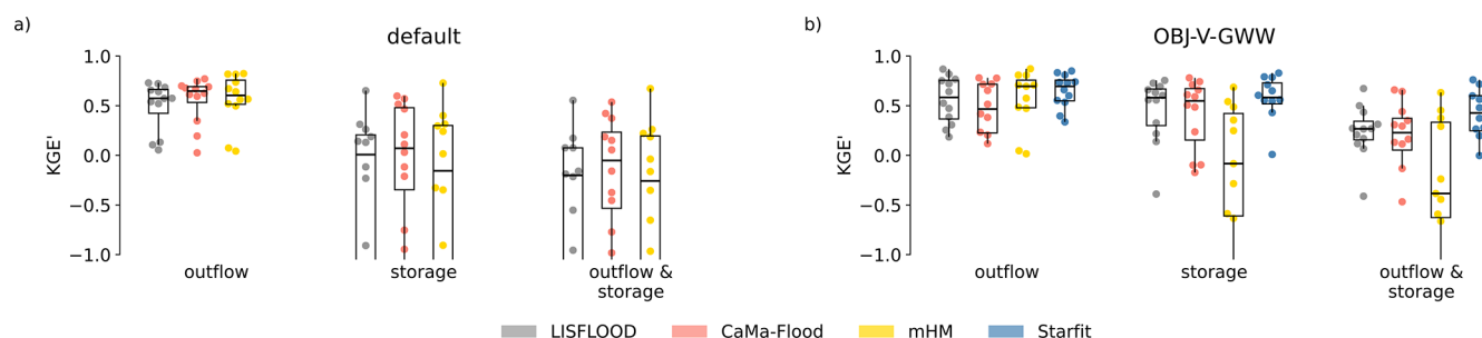
Figure A2. Comparison of model performance across different reservoir routines. The panels represent two experiments: (a) default reservoir parameters, and (b) univariate calibration using reservoir storage estimated by the Global Water Watch (OBJ-V-GWW). Within each panel, three groups of box plots show the performance in terms of outflow, storage, and both variables combined. Four reservoir routines are compared – LISFLOOD, CaMa-Flood, mHM and STARFIT – indicated by colors. The dots represent individual reservoirs, indicating the distribution of overall performance.
