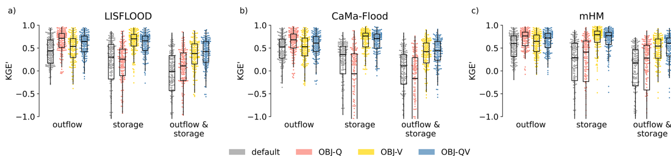
Figure 5. Comparison of the model performance depending on the variable(s) targeted in the calibration. The panels correspond to the three reservoir routines that were calibrated: (a) LISFLOOD, (b) CaMa-Flood and (c) mHM. Within each panel, three groups of box plots show the performance in terms of outflow, storage, and both variables together. Four parameter sets are compared – default parameters, calibration of outflow (OBJ-Q), storage (OBJ-V) and both variables (OBJ-QV) – indicated by colors. The dots represent individual reservoirs, indicating the distribution of the overall performance.
