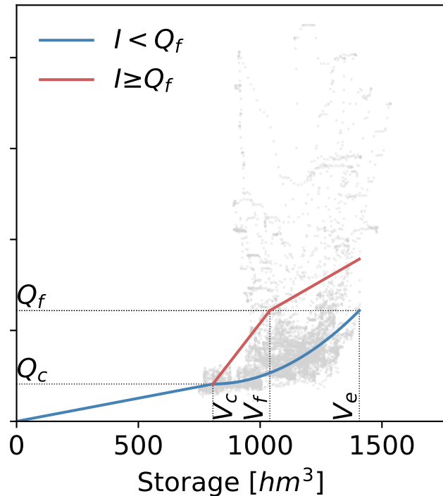
(b) CaMa-Flood
