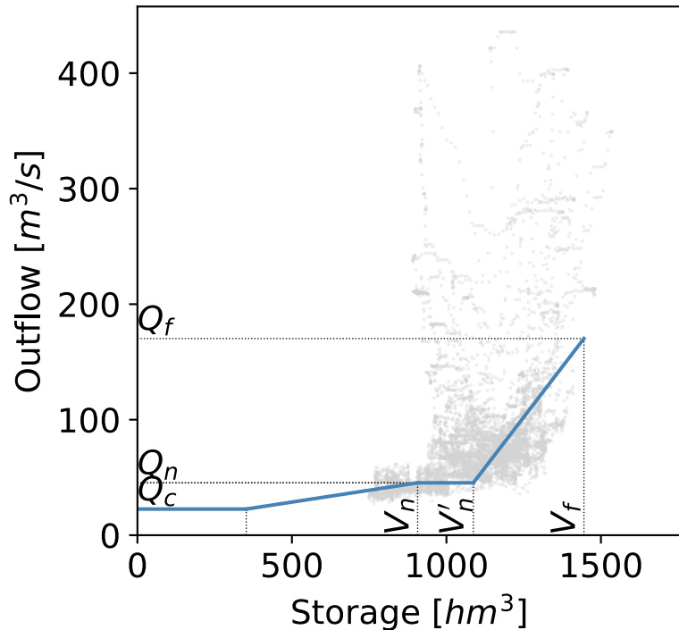
(a) LISFLOOD
