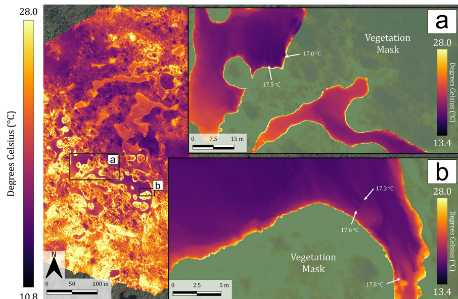
Figure 7. Uncrewed aerial system (UAS) Thermal Infrared (TIR) orthomosaic map of Caribou Bog patterned pools captured on 9 June 2023, and calibrated against the thermal emissivity of water (left, 10.8 to 28.0 °C). Discrete points of cooler water are highlighted (right masked, 13.4 to 28.0 °C) in the (a) the center of the pools and (b) on the upgradient edges of the pools, highlighting localized groundwater discharge hydraulically downgradient in the direction of lateral pool spreading. The resolution of the TIR orthomosaic map is 8.09 cm pixel. Digital basemap data from © Microsoft (2024).
