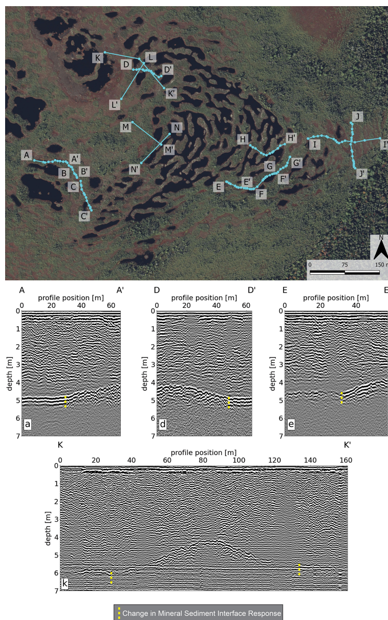
Figure 2. Transects selected from GPR data collected in Thousand Acre Bog (velocity = 0.036 \text{ m ns}^{-1} ), highlighting the changes in the mineral sediment interface reflectors beneath the patterned pools. Basemap data from © Microsoft (2024).
