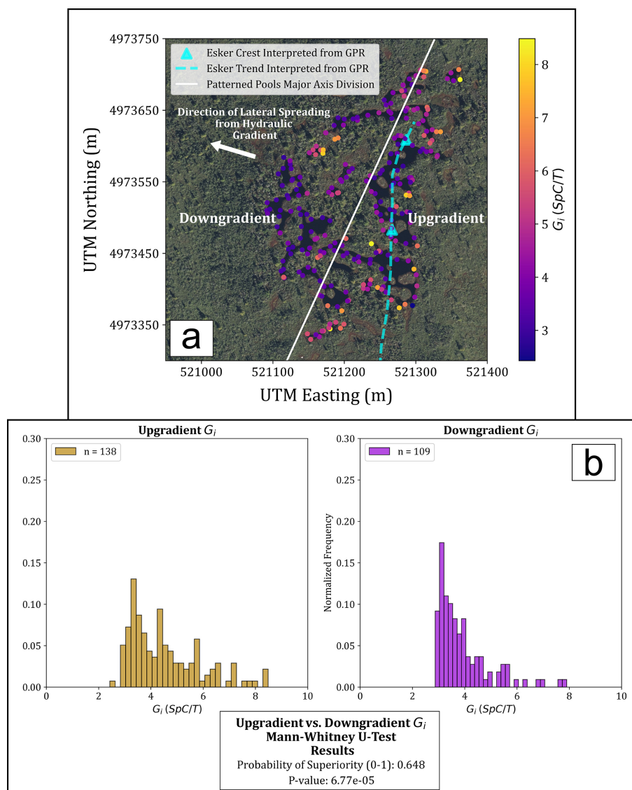
Figure 6. Groundwater indicator ( G_i ) values ( n = 247 ), in (a) given as ratios of specific conductance ( \mu\text{S cm}^{-1} ) to temperature ( ^{\circ}\text{C} ) collected at 0.25 m depth along the perimeter of patterned pools ( n = 13 ) of Caribou Bog (23 and 24 August 2022) with interpreted trends of underlying esker deposits inferred from GPR data, and the inferred direction of lateral spreading for the pool system. Histograms in (b) show the normalized frequency of G_i values of the upgradient and downgradient sections, split by the major axis of the system of patterned pools. In (b), a Mann-Whitney U -Test shows a significant p -value for the difference between the two populations. The probability of superiority demonstrates that the upgradient side of the pools has statistically larger G_i values than the downgradient side of the pools. Basemap data from © Microsoft (2024).
