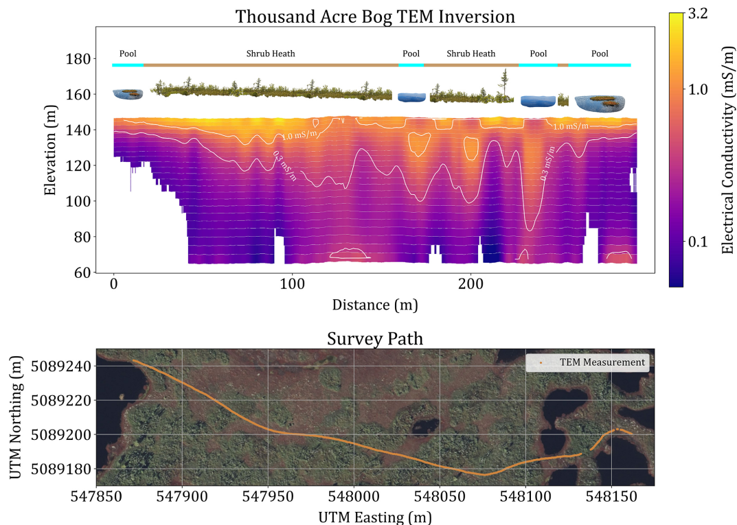
Figure 4. Transient electromagnetic induction (TEM) electrical conductivity ( \text{mS m}^{-1} ) inversion results from surveys conducted in Thousand Acre Bog, indicating variations in the electrical conductivity structures beneath the patterned pools and correspondence to surficial vegetation patterning (Davis and Anderson, 1999). Sensitivity of the TEM inversion was filtered using a standard deviation of less than four to remove low sensitivity portions of the model (white). Basemap data from © Microsoft (2024).
