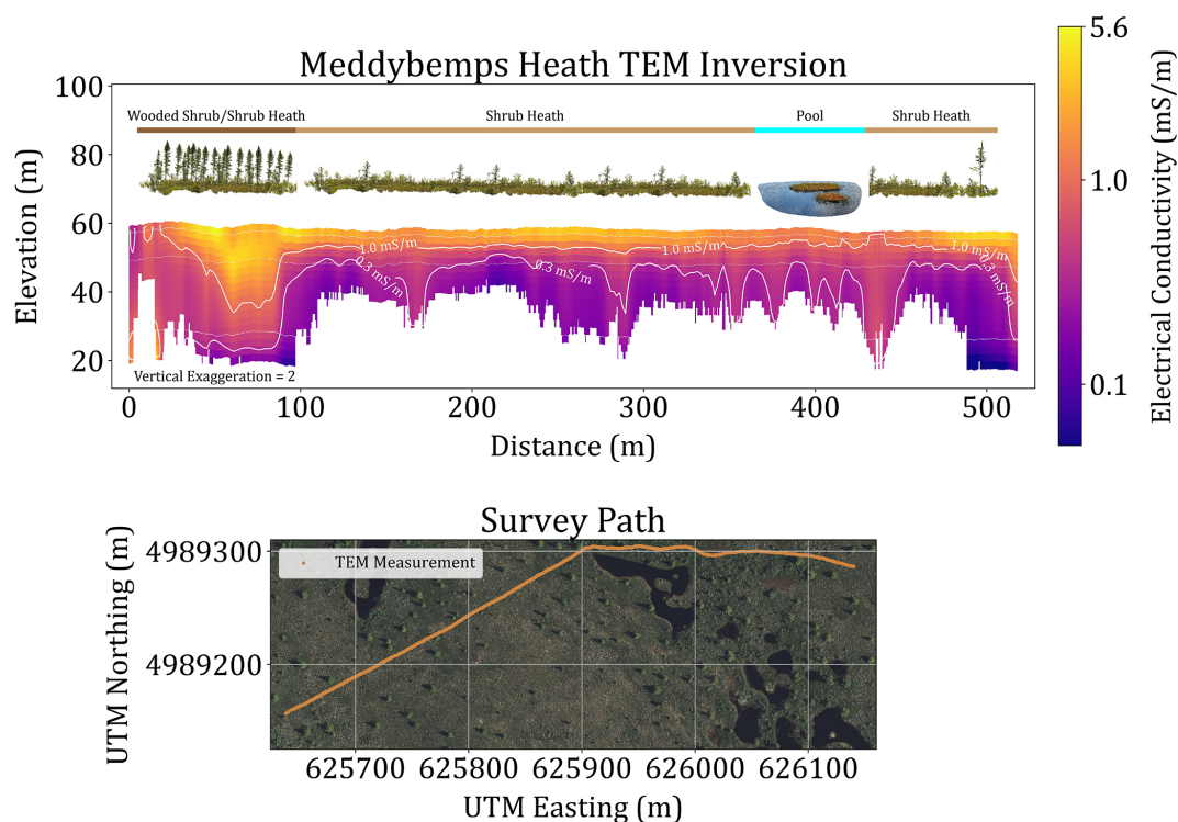
Figure 5. Transient electromagnetic induction (TEM) electrical conductivity ( \text{mS m}^{-1} ) inversion results from surveys conducted in Meddybemps Heath, indicating variations in the electrical conductivity structures beneath the patterned pools and correspondence to surficial vegetation patterning (Davis and Anderson, 1999). Sensitivity of the TEM inversion was filtered using a standard deviation of less than four to remove low sensitivity portions of the model (white). Basemap data from © Microsoft (2024).
