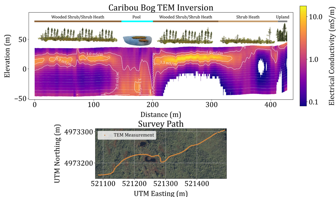
Figure 3. Transient electromagnetic induction (TEM) electrical conductivity ( \text{mS m}^{-1} ) inversion results from surveys conducted in Caribou Bog, indicating variations in the electrical conductivity structures beneath the patterned pools and correspondence to surficial vegetation patterning (Davis and Anderson, 1999). Sensitivity of the TEM inversion was filtered using a standard deviation of less than four to remove low sensitivity portions of the model (white). Basemap data from © Microsoft (2024).
