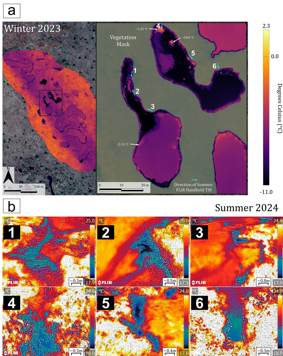
Figure 8. (a) Uncrewed aerial system (UAS) Thermal Infrared (TIR) orthomosaic map of the patterned pools in Meddybemps Heath captured on 3 November 2023, and calibrated against the thermal emissivity of water (top left, -11.0 to 2.3 °C). Points of warmer water highlight the localized discharge of groundwater to the patterned pools moving hydraulically downgradient during the winter season (top right masked, -11.0 to 2.3 °C). Resolution of the TIR orthomosaic map is 19.1 cm pixel and basemap data was retrieved from © Microsoft (2024). (b) Handheld TIR imagery of seepage in Pool 8 imaged facing downgradient (1), imaged facing upgradient (2), imaged facing upgradient (3) and seepage in Pool 9 imaged facing upgradient (4), imaged facing downgradient (5), imaged facing downgradient (6). All imagery was captured on 6 June 2024, at previously established groundwater discharge locations of Meddybemps Heath, highlighting cooler temperature signals during the summer season.
