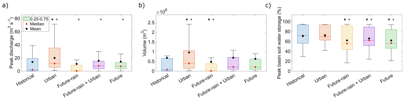
Figure 4. Streamflow peak discharge (a), streamflow volume (b), and peak soil water storage (c) for the four different scenarios compared to the Historical scenario. Box plots are composed of 32 values, where each of these values is the median of 43 spatial shifts for a single storm. Significant differences ( p value < 0.05) between each scenario and the Historical scenario are marked by * for the t -test and by + for the Wilcoxon signed rank test. Similar plots for the other three basins appear in Fig. S2 in the Supplement.
