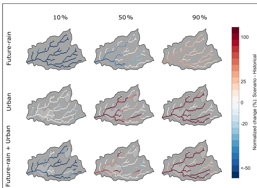
Figure 7. Similar to Fig. 6 but accounting for all storms and spatial rainfall shifts. The columns represent the 10th, 50th, and 90th percentiles of the 32 relative changes computed between each tested rainstorm scenario and the historical benchmark. Similar plots for the other three basins are in Fig. S3 in the Supplement.
