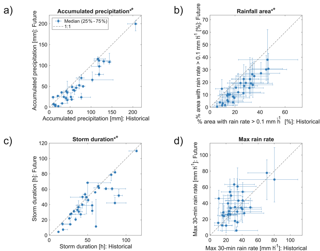
Figure 2. Scatter plots of historical and future rainfall properties for the Dalya basin. Median and 25 %–75 % percentiles across the spatial ensemble are represented by circles and error bars. Significant differences ( p value < 0.05) between the future and historical rainfall are marked by * for the t -test and by + for the Wilcoxon signed-rank test. Similar plots for the other three basins are in Fig. S1 in the Supplement.
