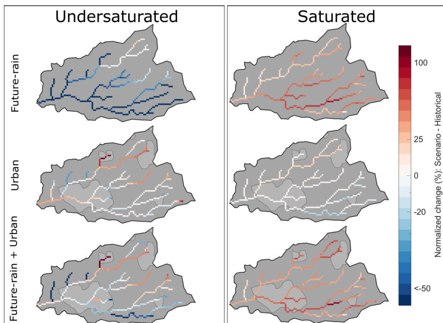
Figure 6. An example of the spatial intra-basin hydrological relative change of different scenarios compared to the Historical one for undersaturated event (left) and saturated event (right). Results show the relative change of peak discharges at each pixel for a single storm shift resulting in the outlet median peak discharge (bold line in Fig. 5). Light gray polygons in the lower two panels represent areas of major projected urbanization changes. Other, less significant land use variations (Fig. 1c), are not represented in this figure. Results for the future scenario are not shown as they are not significantly different from the Future-rain + Urban scenario.
