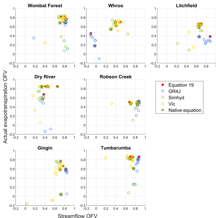
Figure 4. Trade-off plots of objective function values (OFVs) for streamflow ( x -axis) and AET ( y -axis), shown for each catchment. Each subplot displays all 45 calibrations (15 AET equations \times 3 models), with AET equation evap_19 highlighted in red and native AET equations marked with black stars. Higher values indicate better model performance.
