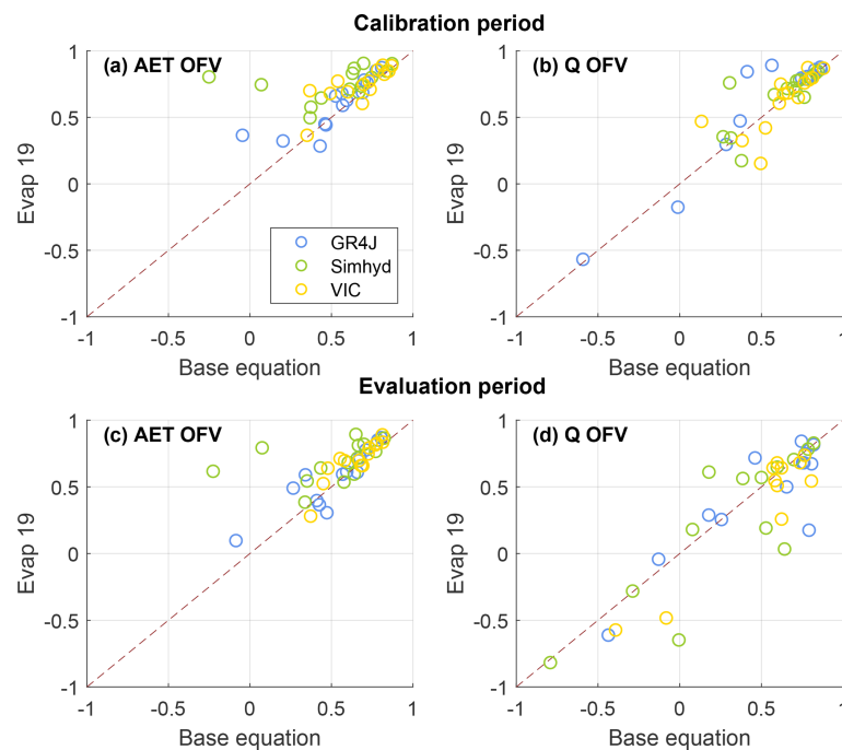
Figure 7. Split-sample test results showing objective function values for AET and streamflow ( Q ). Each point represents a model–catchment combination calibrated on one half of the data and evaluated on the other. Panel figures are as follows: results during the calibration period for AET (a) and streamflow (b), and results during the evaluation period for AET (c) and streamflow (d). Note: Streamflow points with OFVs < -1 under the base equation are omitted.
