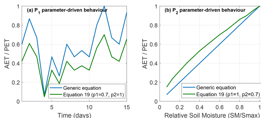
Figure 9. Comparison of equation evap_19 with a typical evapotranspiration formulation (here the generic equation is represented as evap_19 where p_1 and p_2 equal 1). (a) p_1 parameter-driven behaviour: Time series of AET / PET over 15 d, illustrating how evap_19 constrains AET to remain below PET. (b) p_2 parameter-driven behaviour: Relationship between relative soil moisture ( SM/S_{max} ) and AET / PET, showing the stronger non-linear response of AET equation evap_19 to changes in soil moisture availability.
