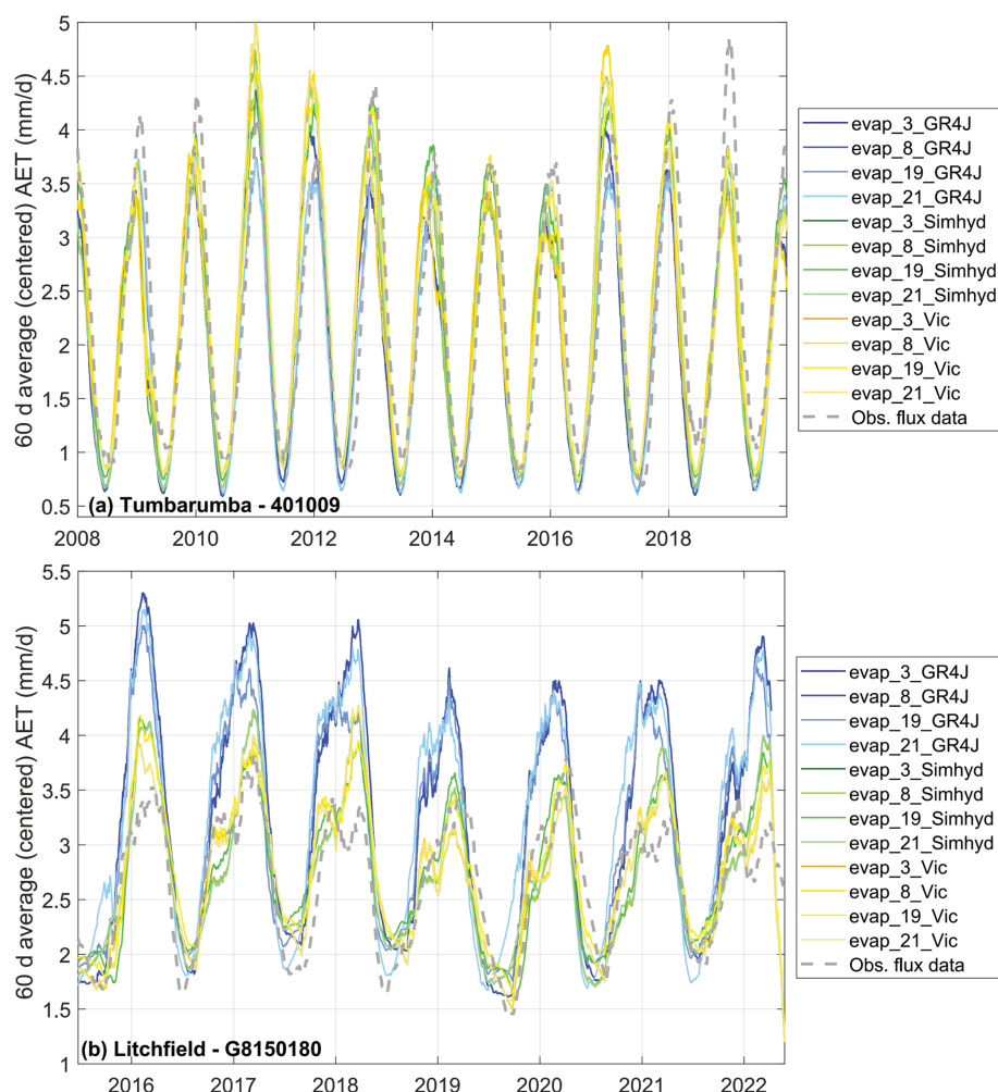
Figure 5. Modelled AET vs. observed flux tower data, showing the four best performing AET equations across the three models at Tumburumba (a) and Litchfield (b).
