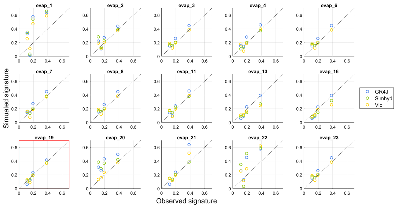
Figure 6. Monthly asynchronicity of AET: observed vs. simulated, across all equations and models. AET equation evap_19 is highlighted with a red box. Remaining signature plots are in the Supplement S6. This signature is purely based on the asynchronicity between normalised PET and AET, calculated by quantifying the area between the normalised curves, and is indicative of seasonal water stress.
