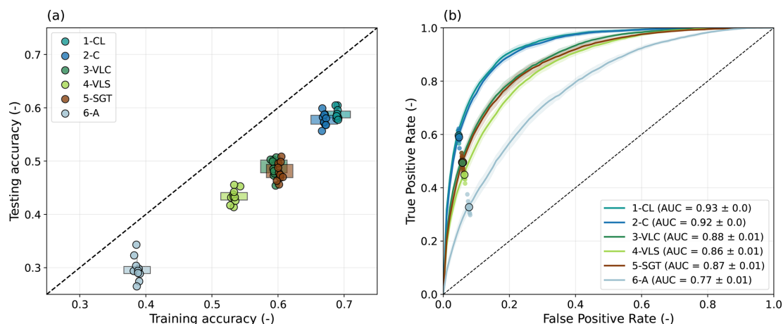
Figure 7. (a) Testing versus training accuracy for each experiment. Each circle represents one of the 10 cross-validation folds. The axes are extended slightly beyond the data range to show the 1 : 1 reference line. Boxplots beneath the points summarise the distribution of testing accuracies across the 10-fold cross-validation for each experiment. (b) The averaged ROC curves for each experiment are displayed, computed over the 10 cross-validation folds. For each fold, the true positive rate ( R_{TP} ) and false positive rate ( R_{FP} ) at the actual classification threshold are shown as small dots. The larger dot represents the average R_{TP} and R_{FP} across all folds, corresponding to the aggregated performance reported in the confusion matrices.
