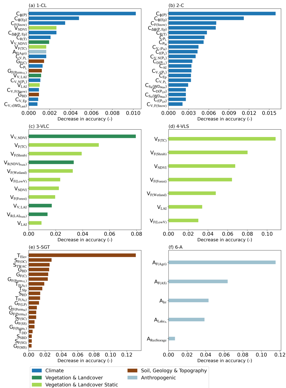
Figure 10. Median feature importance across the 10-fold cross-validation for all six experiments. Features are ranked by importance (y-axis), which is dictated by the decrease in model accuracy ( \text{Acc}_{\text{test}} ) by removing the corresponding attribute (x-axis). Panels (a), (b) and (e) display only the 20 most important features. Feature importance values are not directly comparable across experiments because they depend on the model type and the number and composition of input features; experiments with fewer predictors typically yield higher importance values per feature.
