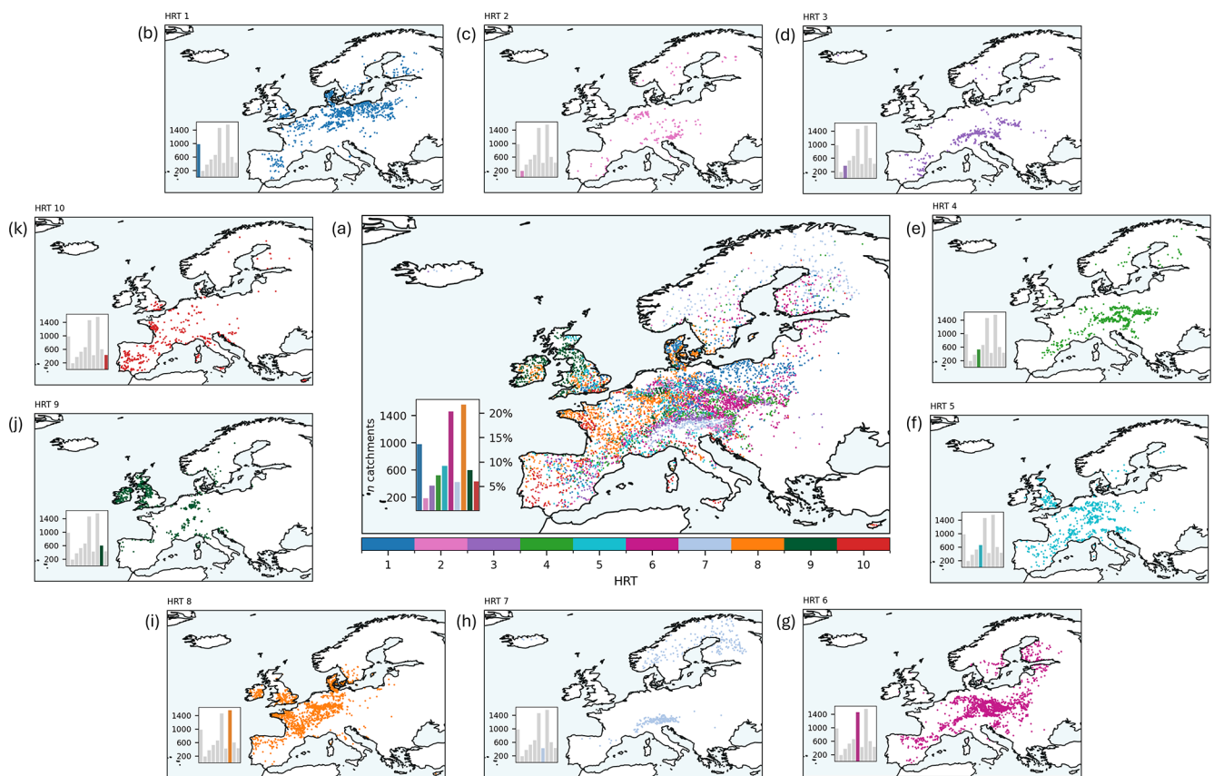
Figure 6. Classification of 7175 catchments into 10 HRT based on 40 hydrological signatures. The HRTs are ordered by increasing slope of the flow duration curves. Panel (a) presents all HRTs together, panels (b) to (k) show the spatial distribution of each HRT individually.
