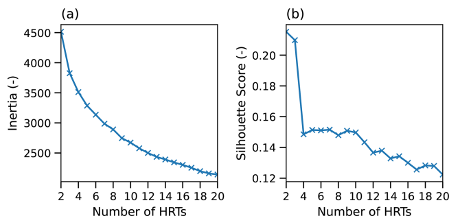
Figure 2. Assessment of cluster robustness using k -means clustering. (a) Elbow Method results for k = 2 –20 HRTs, used to evaluate the optimal number of hydrological response types. (b) Silhouette Scores for the same range of HRTs, providing an additional metric of cluster cohesion and separation.
