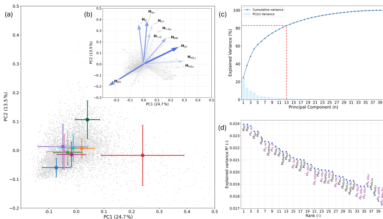
Figure 3. Principal Component Analysis (PCA) of the 40 hydrological signatures across the HRTs. (a) Explained variance of PC1 (24.7 %) and PC2 (13.5 %) for each catchment (grey), with HRT means and standard deviations shown in their respective colour. (b) Loadings of the hydrological signatures, shown for PC1 and PC2. Arrow thickness and colour intensity reflect each signature's ranked explained variance based on the first 13 PCs (see panel d ), accounting for just above 80 % of the cumulative explained variance. Thicker and more intense coloured arrows indicate more informative signatures. (c) Cumulative explained variance across all principal components. The explained variance of the first 13 PCs is highlighted by the red dashed lines. (d) Ranked explained variance of the first 13 PCs, which together account for approximately 80 % of the total variance. Signatures related to variance are highlighted in purple.
