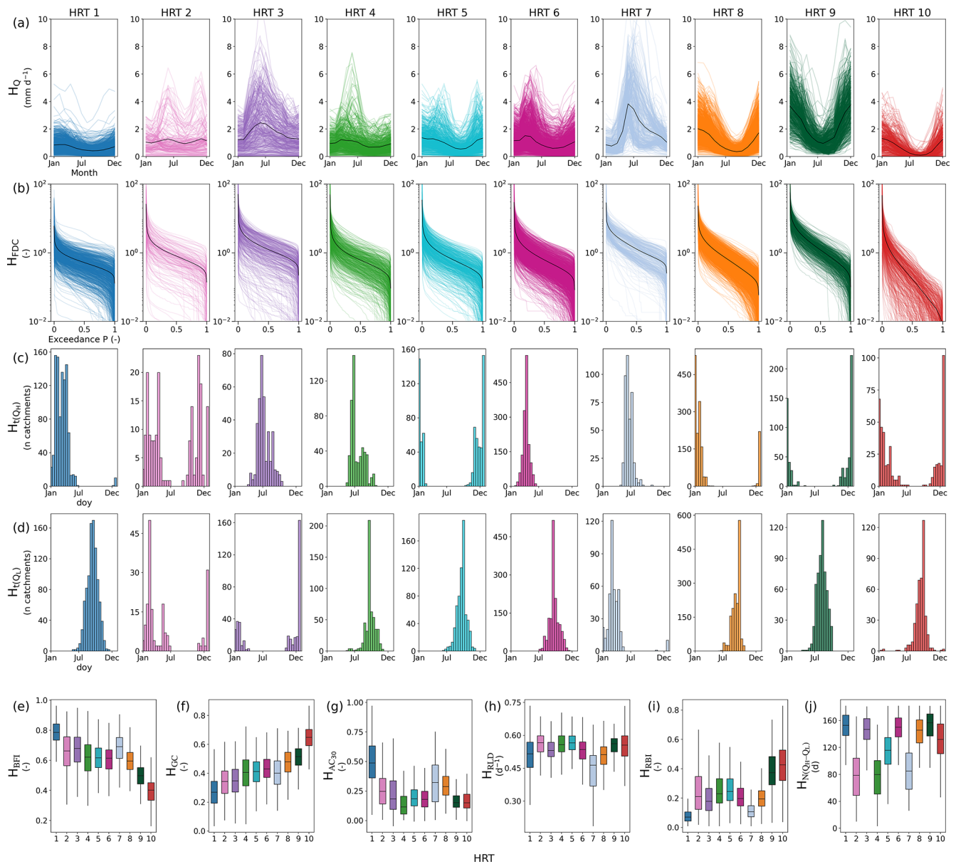
Figure 4. Visualisation of 10 out of the 40 hydrological signatures across hydrological response types (HRTs), the remaining 30 signatures can be seen in Fig. S2. Panels (a)–(d) show four selected signatures for each HRT (one row per signature, one column per HRT), (a) streamflow ( H_Q ), (b) flow duration curves ( H_{FDC} ), (c) high flow timing ( H_{t(Q_H)} ) and (d) low flow timing ( H_{t(Q_L)} ), highlighting within- and between-cluster variability. In panels (a) and (b), the black line indicates the mean value of mean discharge ( Q ) and mean flow duration curve (FDC), respectively. Panels (e)–(j) display boxplots of six additional hydrological signatures, (e) baseflow index ( H_{BFI} ), (f) Gini coefficient ( H_{GC} ), (g) autocorrelation ( H_{AC_{30}} ), (h) rising limb density ( H_{RLD} ), (i) flashiness index ( H_{RBI} ) and (j) days between highest and lowest flow ( H_{N(Q_H-Q_L)} ), summarising their distribution across HRTs.
