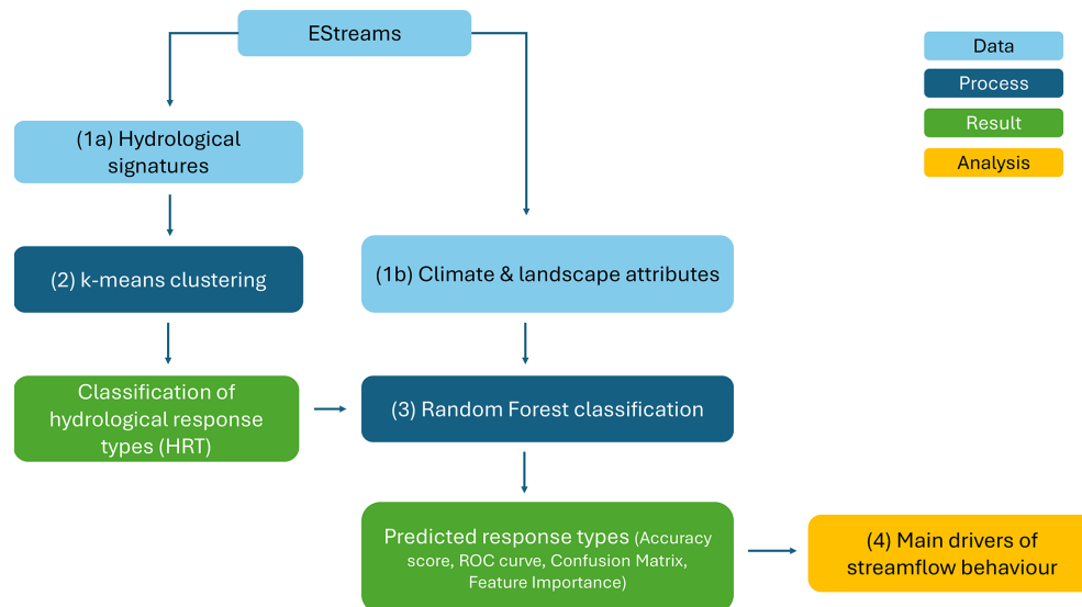
Figure 1. Workflow of the study. Streamflow time series and catchment attributes (1) were used to classify hydrological response types (HRT) to the individual catchments via k -means clustering (2) and predict HRT membership using a Random Forest classification model (3). The importance of individual attributes was quantified from the Random Forest classification model to identify the dominant controls on HRT membership and thus the main drivers of the hydrological response (4).
