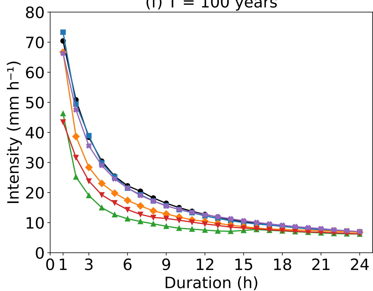
(f) T = 100 years
