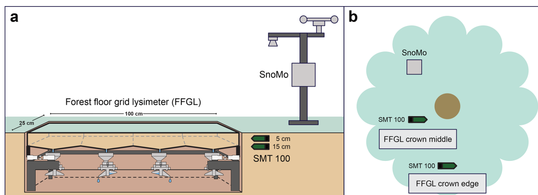
Figure 1. Installed setup (a) containing a microclimate station (SnoMo), soil moisture probes (SMT100) and forest floor grid lysimeters (FFGL), and (b) the corresponding positioning to the tree.
