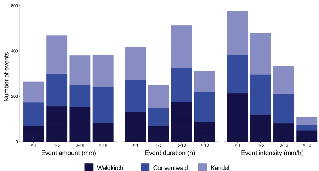
Figure 5. Measured throughfall amount, intensity and duration of the observed events.
