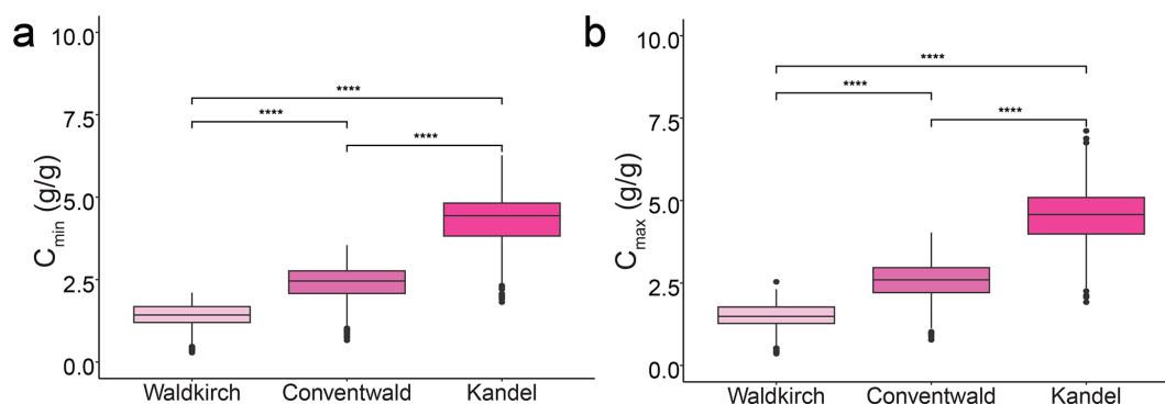
Figure 7. Mean minimum (a) and maximum (b) water holding capacity ( C_{\min} and C_{\max} ) on the three different research sites. Overlaid significance symbols indicate the results of statistical t-tests between the sites. The significance levels are represented as follows: **** ( p \leq 0.0001 ).
