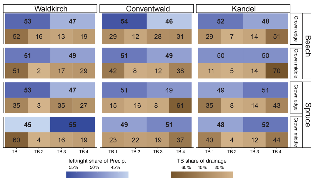
Figure 10. Percentage share of precipitation (blue) on the left/right site of the lysimeter in relation to the field setup, bold numbers show a significant difference (t-test), and infiltration distribution (brown), showing the ability of the FF to redistribute water fluxes.
