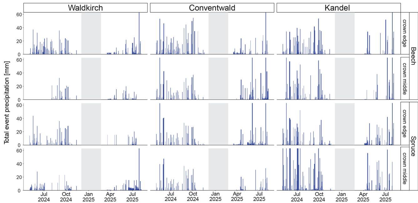
Figure 4. Identified rainfall events and their total Throughfall ( P_{TF} ) for all twelve lysimeters, the snow-affected period which was excluded from the statistical analysis is rendered in grey.
