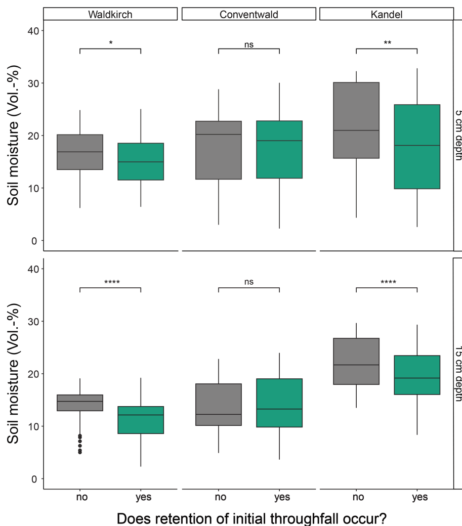
Figure 6. Tendency for throughfall retention to occur in relation to soil moisture at 5 and 15 cm depth. No = There is no retention occurring in the first interval of an event, yes = retention occurs during the first interval (10 min) of the event. We found a significant difference in soil moisture leading to initial throughfall retention or not in Waldkirch and at Kandel. Retention usually occurs with lower soil moisture contents. Overlaid significance symbols indicate the results of statistical t-tests between the groups. The significance levels are represented as follows: * ( p \leq 0.05 ), ** ( p \leq 0.01 ), *** ( p \leq 0.001 ), **** ( p \leq 0.0001 ), and ns ( p > 0.05 )
