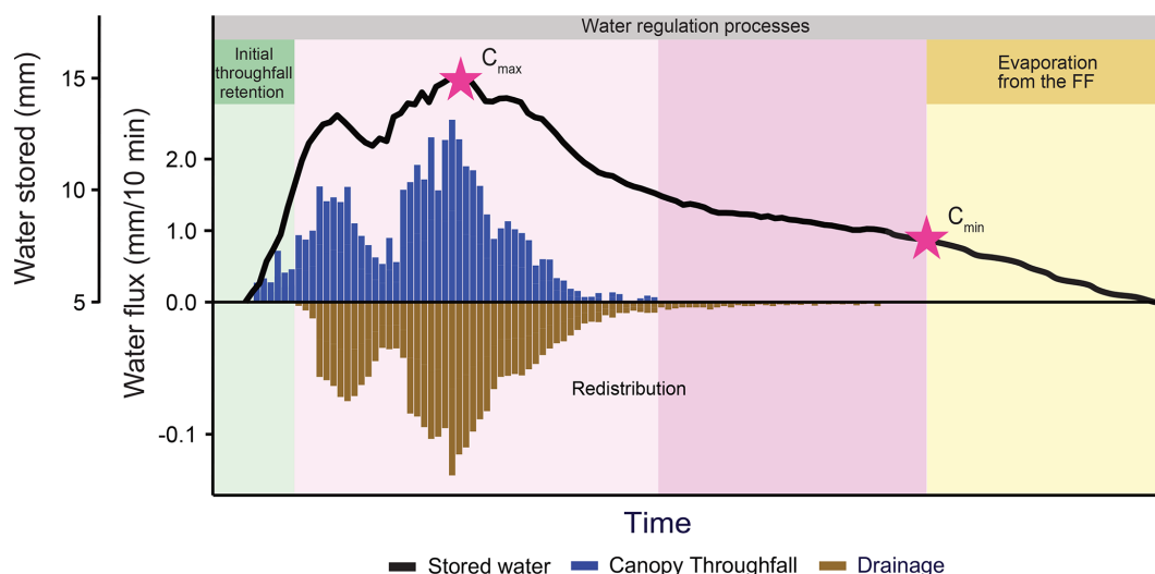
Figure 2. Exemplary run of one precipitation event, including precipitation and drainage amount as well as the progression of lysimeter weight, showing the different phases initial throughfall retention, storage, redistribution and evaporation.
