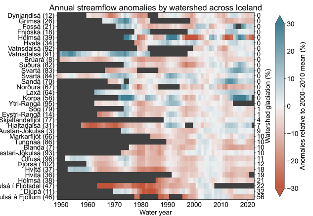
Figure 2. Annual streamflow anomalies for Icelandic gauges with extended measurement records. Anomalies are expressed as percentages relative to each gauge’s mean streamflow during the common reference period (1 October 2000 to 30 September 2010), allowing for direct comparison across catchments. A 5-year centered rolling average is applied to smooth short-term variability. The color scale indicates percentage anomalies, with red representing below-average flows and blue representing above-average flows relative to the reference period. The left y-axis lists river names and corresponding LamaH-Ice gauge IDs, while the right y-axis displays catchment glaciation percentages.
