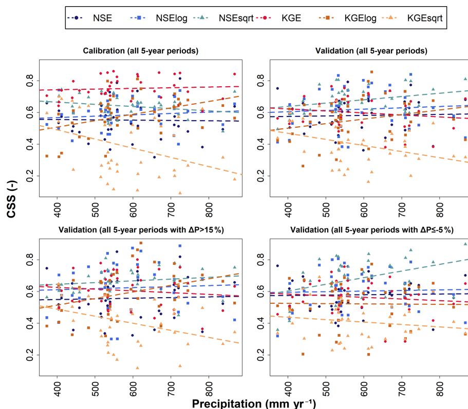
Figure 2. Scatterplots with the composite scaled score (CSS) of the parameterizations obtained with each of the six objective functions for 38 watersheds ( y -axis), plotted against the long-term average annual precipitation of the watersheds ( x -axis). The dashed lines represent the linear trend between CSS and precipitation per objective function.
