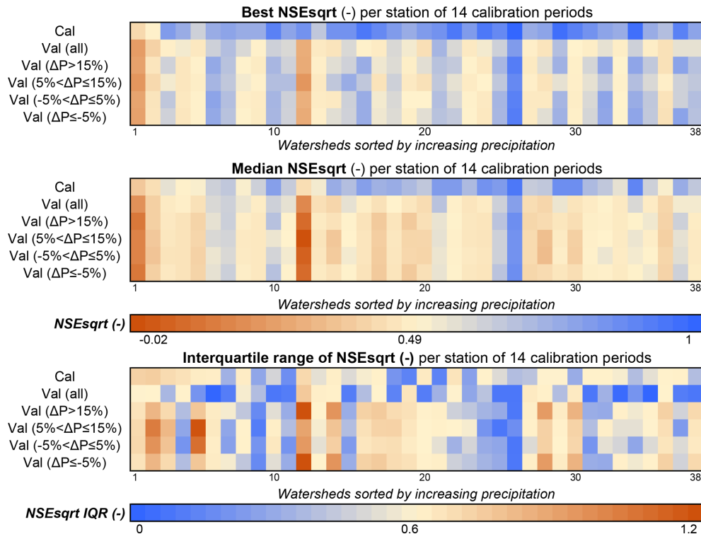
Figure 3. Heatmap with the best (top), median (middle) and interquartile range (IQR) (bottom) of NSEsqr (–) for each watershed, sorted by increasing long-term annual average precipitation (columns) and each calibration-validation set of runs (rows). The values of NSEsqr or the IQR for each cell in the heatmap are computed as averages of the values from the 14 5-year calibration runs, the 13 validation runs for each of the 14 calibration runs. i.e., Val (all), and the validation runs corresponding to each of the four precipitation change classes, as specified in Table 1.
