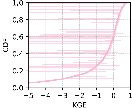
BM14 Monthly RRR to daily P
