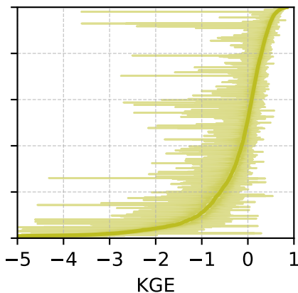
BM15 Scaled P
