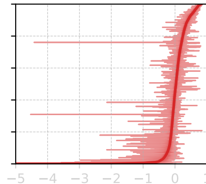
BM13 Monthly RRR to monthly P
