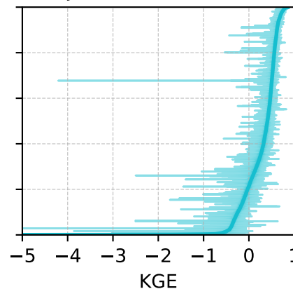
BM17 Adjusted Smoothed P
