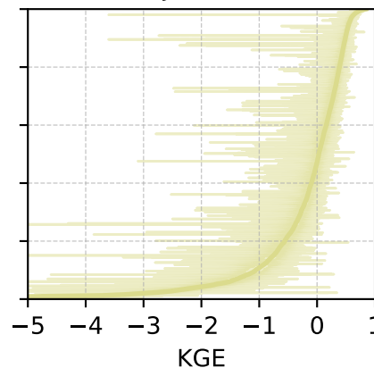
BM16 Adjusted P
