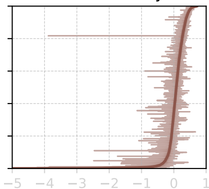
BM11 RRR to monthly P
