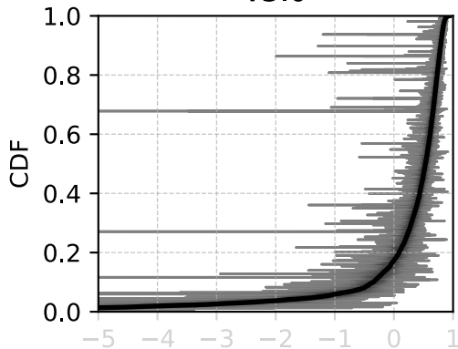
BM08 Daily median flow
