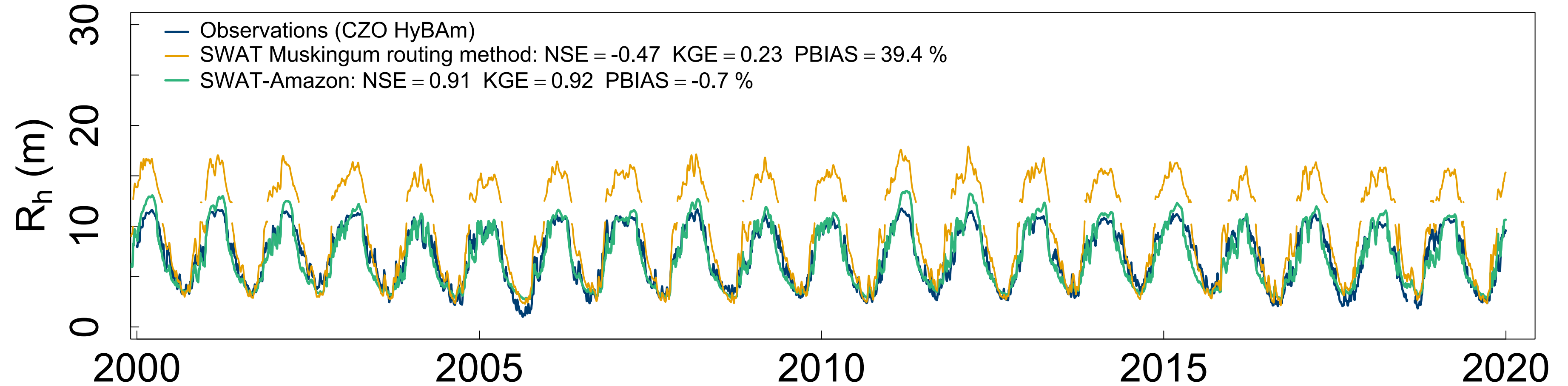
(a) Water Level or Hydraulic Radius
