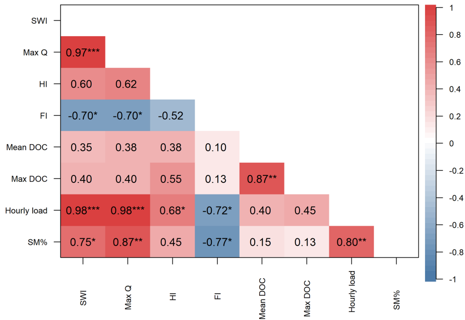
Figure 7. Correlation matrix for mean SAGA wetness index (SWI), maximum discharge (Max Q ), hysteresis index (HI), flushing index (FI), mean and maximum DOC concentration, hourly DOC load, and daily meltwater contribution (SM %). Significant correlations are flagged, * for p < 0.05 and *** for p < 0.001 .
