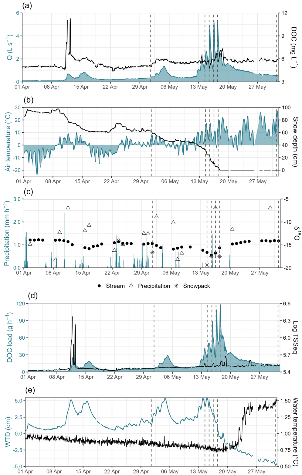
Figure 4. Water quality and hydrological parameters monitored during the study period April–May. Discharge ( Q ) and DOC concentration monitored at the stream gauging station (a), air temperature and automatic point snow depth measurement in Puukkosuo (b), precipitation monitored in Puukkosuo and \delta^{18}O isotope samples of the stream, precipitation, and snow (c), DOC load and TSSeq concentration (d), and water table depth (WTD) and water temperature monitored in the GW well in Puukkosuo (e). Dashed lines represent the dates of UAS surveys.
