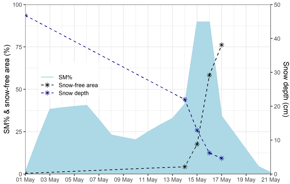
Figure 5. The estimated daily meltwater contribution (SM %) during the peak melt period (1–20 May) based on isotope hydrograph separation, mean snow depth (cm), and snow-free area (%) obtained from the UAS surveys.
