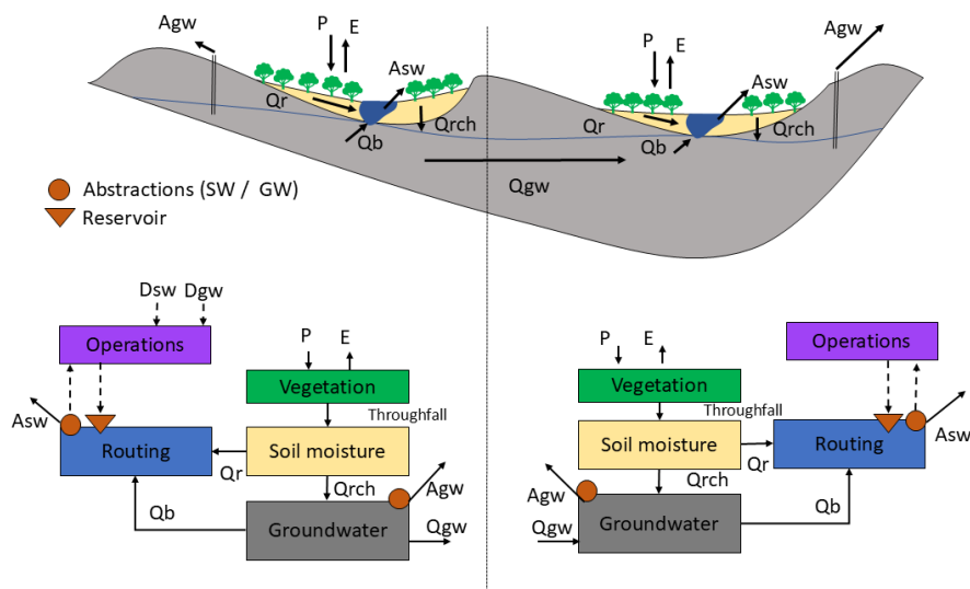
Figure S1. Schematic cross-section of atmospheric, surface and sub-surface fluxes with water management interventions and operations in a groundwater-rich area. Shown fluxes include precipitation ( P ), evaporation ( E ), runoff ( Q_r ), baseflow ( Q_b ), groundwater recharge ( Q_{rch} ), lateral groundwater flow ( Q_{gw} ), demand for surface water ( D_{sw} ) and groundwater ( D_{gw} ) and abstractions for surface water ( A_{sw} ) and groundwater ( A_{gw} ).
