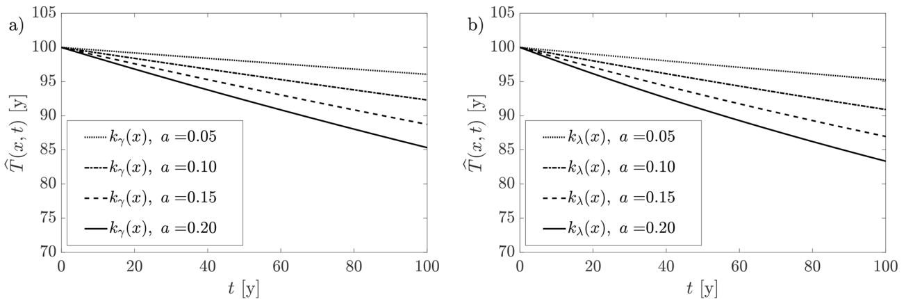
Figure 5. The value of the initial stationary return period \bar{T}_0(x) = 100 y varies in time (future timeframe, t ) due to a linear trend in the Gumbel distribution, for different values of the parameter a of the weakly non-stationary framework (Eq. 8). The linear trend in \gamma(t) , k_\gamma , is given by Eq. (22). The linear trend in \lambda(t) , k_\lambda , is given by Eq. (23). (a) Time-varying return period with a linear trend in \gamma(t) ; (b) Time-varying return period with a linear trend in \lambda(t) .
