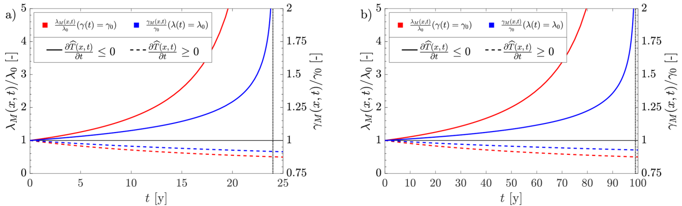
Figure 4. The simplified solution of Eqs. (20) and (19) in case the trend affects one parameter at a time. Both the solutions for decreasing (solid line) and increasing (dashed line) return period at different future timeframes, t , are shown ( a = 1 in both the panels). The plots refer to two different values of the initial return period: (a) \bar{T}_0(x) = 25 y; (b) \bar{T}_0(x) = 100 y. In both the panels, the vertical asymptote represents the limit condition t = \frac{\bar{T}_0(x) - \Delta\tau}{a} , which is equal to t = \bar{T}_0(x) - 1 for \Delta\tau = 1 year and a = 1 .
