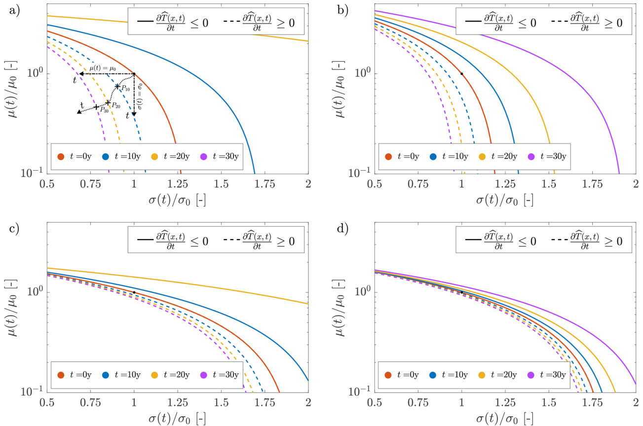
Figure 2. The graphical behavior of Eq. (13) at varying the initial return period, \bar{T}_0(x) , for the Fréchet (panel a and b ) and the Weibull (panel c and d ) distributions at different future timeframes, t , for both the cases of decreasing (solid line) and increasing (dashed line) return period. The black dot highlights the initial condition in all the panels. In panel (a) , dashed-dotted black lines show time evolution for the trend in one single parameter (Eqs. 14 and 15), and the dotted black line shows a general trend in both the parameters, for the case of increasing return period. The points P_t identify the limit solution at time t along the trend line. a = 1 in all the panels. (a) Fréchet distribution, \bar{T}_0(x) = 25 y; (b) Fréchet distribution, \bar{T}_0(x) = 50 y; (c) Weibull distribution, \bar{T}_0(x) = 25 y; (d) Weibull distribution, \bar{T}_0(x) = 50 y; (b) \bar{T}_0(x) = 50 y. In panels (a) and (c) , the continuous violet line does not satisfy the condition t \leq \frac{\bar{T}_0(x) - \Delta\tau}{a} , and therefore it is not shown.
