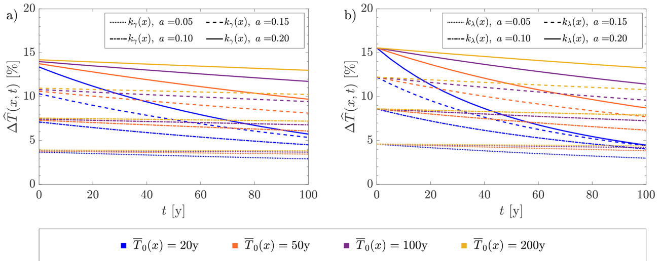
Figure 7. The degree of approximation (Eq. 21) of the proposed framework at varying the initial return period, \bar{T}_0(x) and the parameter a , for the cases of linear trend in the mean magnitude ( k_\gamma(x) , Eq. 22, panel a) and mean frequency ( k_\lambda(x) , Eq. 23, panel b).
