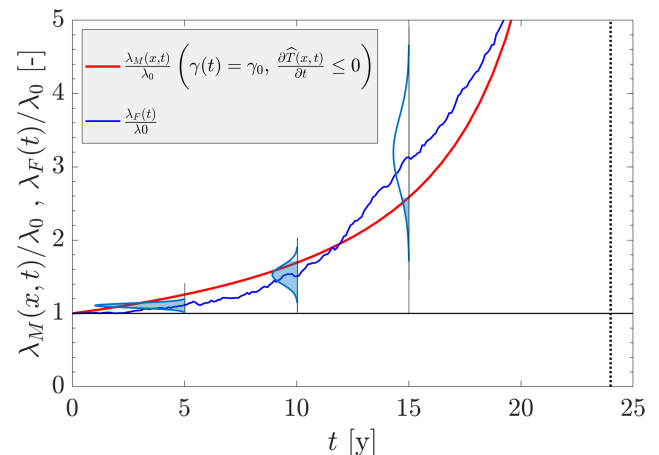
Figure 6. A comparison between the limit solution (red line) for \lambda_M(x, t) (Eq. 20, with a = 1 and \bar{T}_0(x) = 25 y) and a hypothetically-forecasted trend, \lambda_F (blue line), with the uncertainty estimation given by the pdf (light blue curves). At each future timeframe t , there is a probability (shaded area in each pdf) that the forecasted trend satisfies the weakly-nonstationary condition (i.e., \lambda_F(t) \leq \lambda_M(x, t) ).
