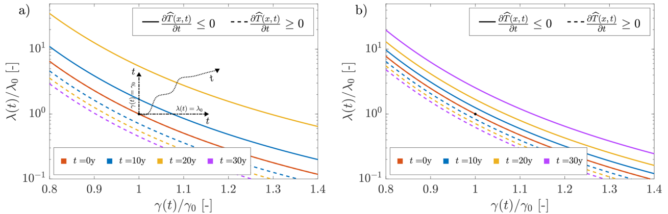
Figure 3. The graphical behavior of the limit solution for the Gumbel distribution (Eq. 18) at different future time horizons, t , for both the cases of decreasing (solid line) and increasing (dashed line) return period. The black dot highlights the initial condition in both panels ( \lambda_0 = 73 , \gamma_0 = 50 ). In panel (a), dashed-dotted black lines show time evolution for the trend in one single parameter (Eqs. 19 and 20), and the dotted black line shows a general trend in both the parameters, for the case of decreasing return period. a = 1 in all the panels. The panels refer to two different values of the initial return period: (a) \bar{T}_0(x) = 25 y; (b) \bar{T}_0(x) = 50 y. In panels (a), the continuous violet line does not satisfy the condition t \leq \frac{\bar{T}_0(x) - \Delta\tau}{a} , and therefore it is not shown.
