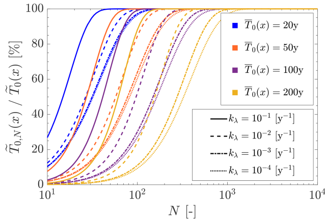
Figure 8. A comparison between the approximated solution of Eq. (2) with N terms, \tilde{T}_{0,N}(x) , and the actual solution, \tilde{T}_0(x) , according to different combinations of initial stationary return period, T_0(x) , and linear trend coefficient in the mean frequency, k_\lambda , of a Poisson Process with initial mean frequency, \lambda_0 = 73 \text{ y}^{-1} .
