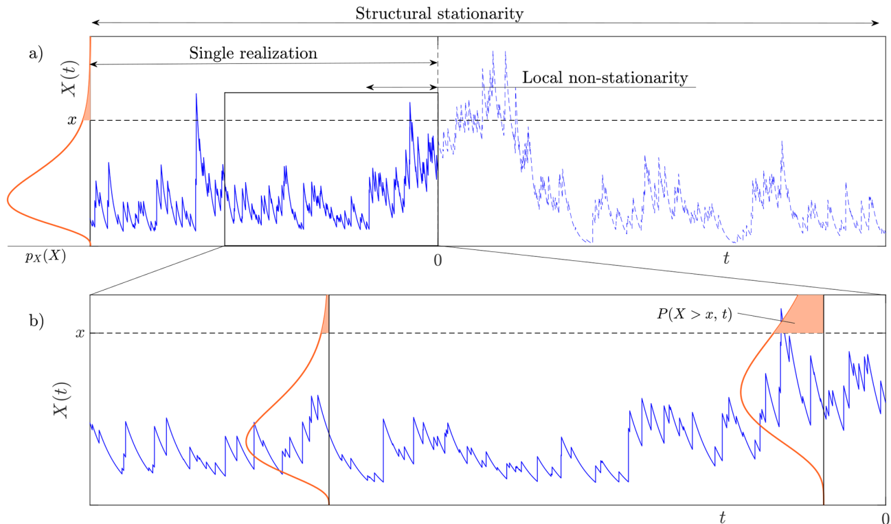
Figure 1. A sample realization of a structurally stationary Poisson-based stochastic process with constant parameters (mean frequency between events and mean jump magnitude) showing a local non-stationarity of long duration (continuous blue line) appearing up to the observation time ( t = 0 y, present day). Dashed blue line represents a potential (unknown) future evolution of the process. Orange curves and shaded areas are the stationary, p_X(X) , and non-stationary, p_X(X, t) , pdfs and the cumulative probability, P(X > x, t) , above the threshold x (dashed black line), respectively. (a) A Compound Poisson Process with linear drift as a proxy for flow discharges in a river. Structural (long-term) stationarity is foreseen, but local non-stationarity arises in the short term. b) The cumulative probability above the threshold x changes when calculated according to short-term properties of the system's dynamics.
