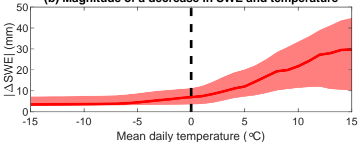
(b) Magnitude of a decrease in SWE and temperature
