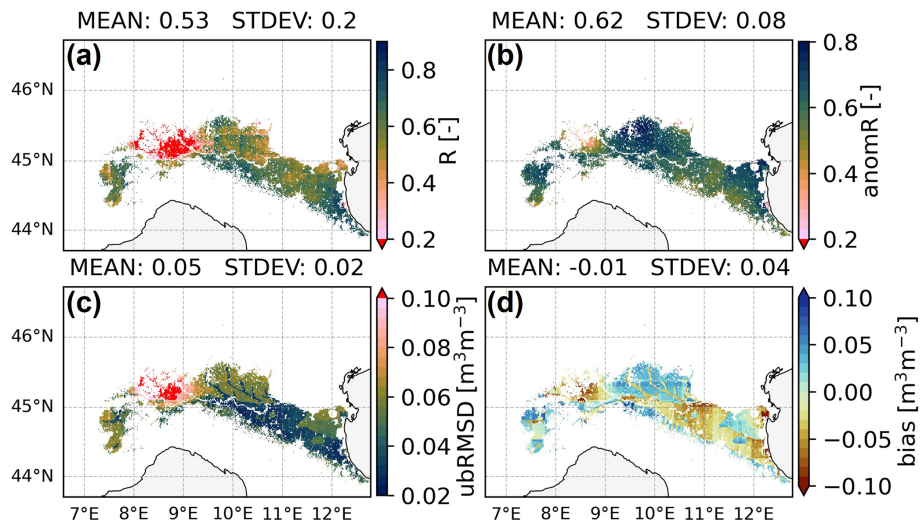
Figure D1. Maps of R [-], \text{anom}R [-], \text{ubRMSD} [ \text{m}^3 \text{m}^{-3} ], and \text{bias} [ \text{m}^3 \text{m}^{-3} ] of the evaluation of AquaCrop 15 d SSM estimates against SMAP 1 km SSM for March through September.
