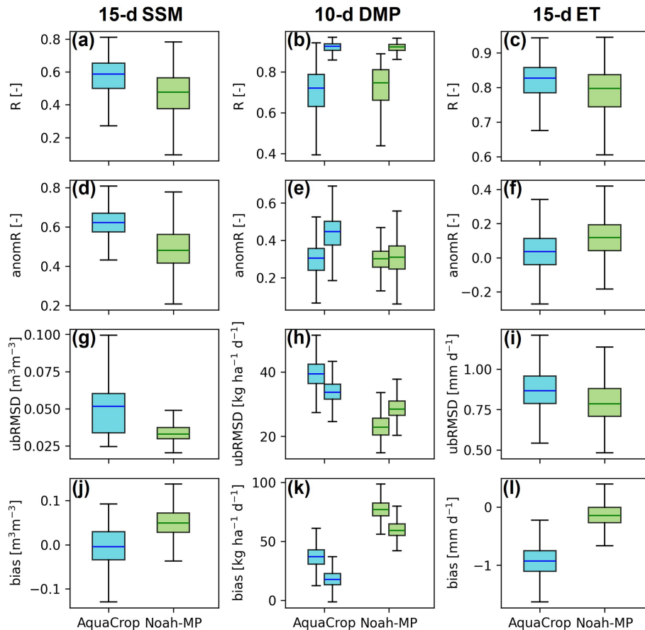
Figure 4. Boxplots of R , ubRMSD, anom R , and bias of AquaCrop (blue) and Noah-MP (green) simulations, comparing (i) modeled SSM with SMAP SSM, (ii) modeled vegetation with CGLS DMP, (iii) modeled ET with SenET. Metrics were computed for the months March through September 2015–2022 for SSM and vegetation, and the same months but 2017–2021 for SenET. For the evaluation with CGLS DMP, the second boxplot presents the metrics computed for the months from January through June 2015–2022.
