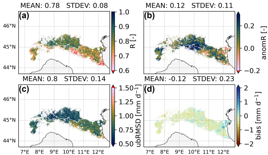
Figure F2. Maps of R [-], \text{anom}R [-], \text{ubRMSD} [ \text{mm d}^{-1} ], and \text{bias} [ \text{mm d}^{-1} ] of the evaluation of Noah-MP 15 d ET estimates against SenET for March through September.
