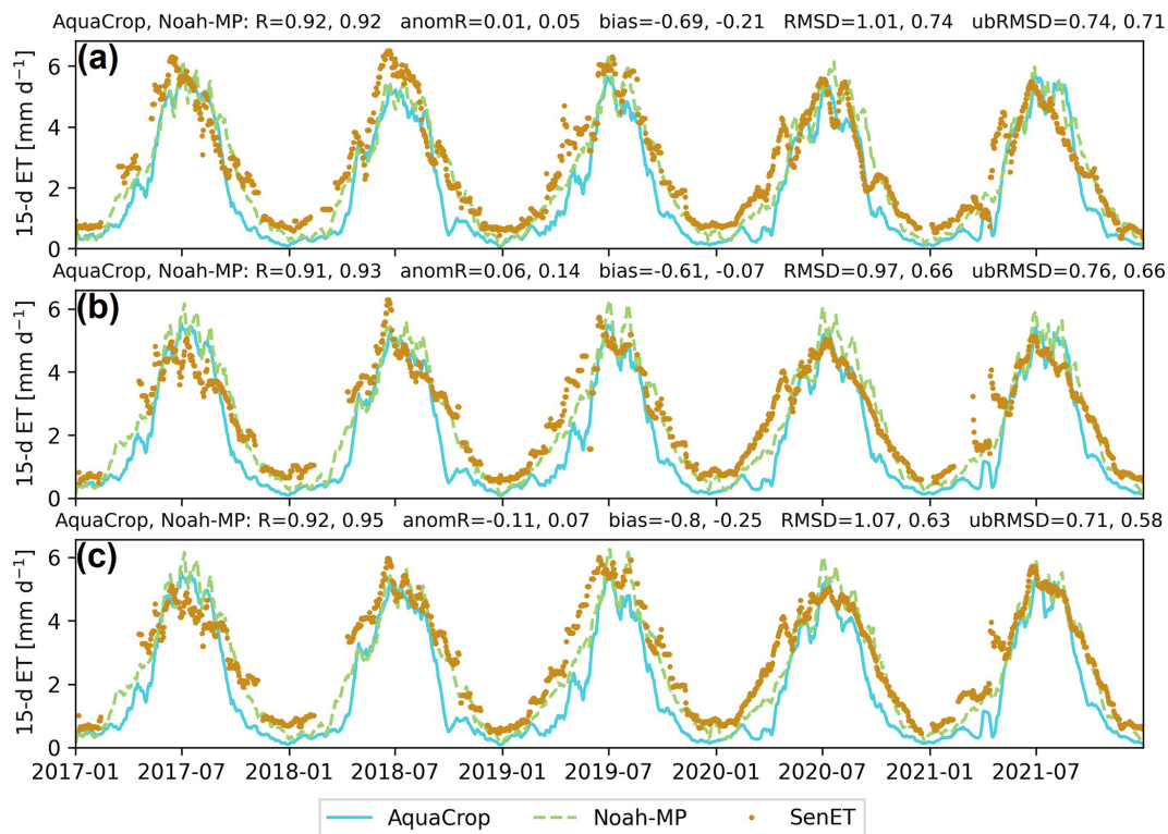
Figure G1. Time series of AquaCrop and Noah-MP 15 d ET estimates along with SenET retrievals for (a) Budrio (1 pixel), (b) Faenza San Silvestro (3 pixels), and (c) Faenza Formellino (8 pixels). The metrics are computed over the full year.
