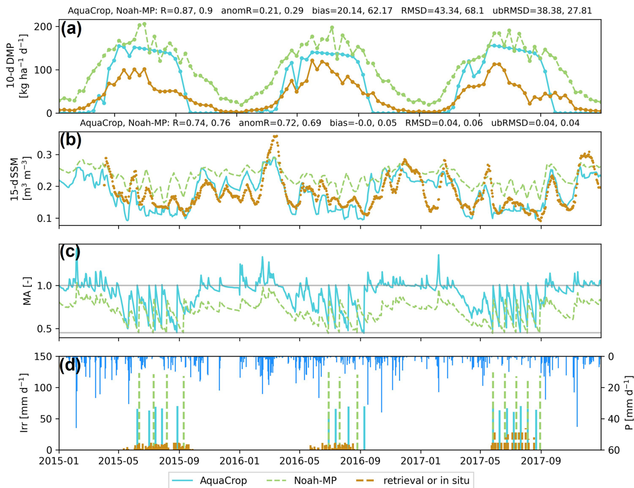
Figure 6. Time series of different variables for AquaCrop (full blue lines), Noah-MP (dashed green lines), and reference data (dashed ochre lines and points) at the Budrio site. (a) 10 d DMP [ \text{kg ha}^{-1} \text{d}^{-1} ] of both models and CGLS DMP. (b) 15 d SSM [ \text{m}^3 \text{m}^{-3} ] from both models and SMAP. (c) moisture availability (MA [-]). (d) irrigation from both models and field data [ \text{mm d}^{-1} ] (left y axis) and precipitation [ \text{mm d}^{-1} ] from MERRA2 (right reverted y axis). For a and b, the metrics of both model estimates against the reference are shown in the title.
