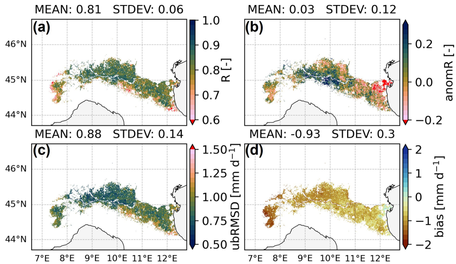
Figure F1. Maps of R [-], \text{anom}R [-], \text{ubRMSD} [ \text{mm d}^{-1} ], and \text{bias} [ \text{mm d}^{-1} ] of the evaluation of AquaCrop 15 d ET estimates against SenET for March through September.
