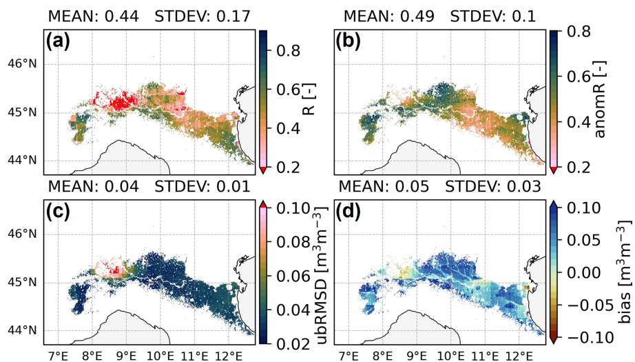
Figure D2. Maps of R [-], anomR [-], ubRMSD [ m^3 m^{-3} ], and bias [ m^3 m^{-3} ] of the evaluation of Noah-MP 15 d SSM estimates against SMAP 1 km SSM for March through September.
