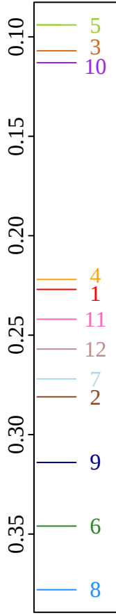
Baseflow index [-]
