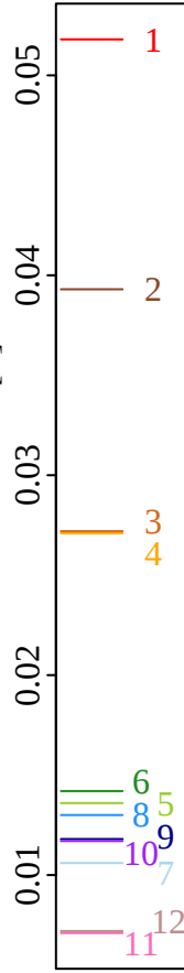
Flashiness index [-]
