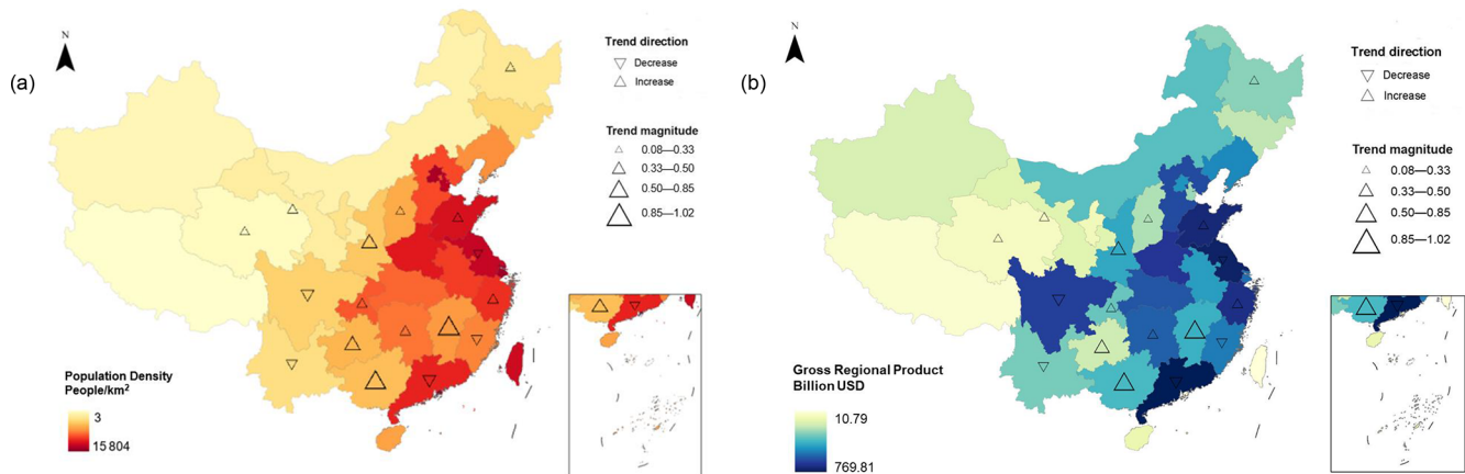
Figure 7. The analysis of flood event trends across the Chinese provinces from 2000 to 2022, shown in relation to (a) population density and (b) gross regional product (GRP). The triangles indicate trends: downward triangles represent decreases, and upward triangles represent increases, with the sizes corresponding to the trend values. Publisher's remark: please note that the above figure contains disputed territories.
