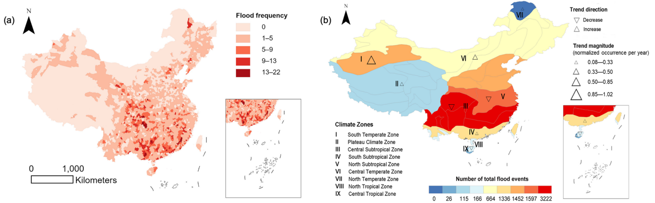
Figure 6. Spatial distribution of flood occurrences and trends in China (2000–2022). (a) The accumulated flood occurrences at the county level. (b) The accumulated flood occurrences and trends across different climate zones, where Roman numerals denote the climate zones. The triangles indicate trends: downward triangles represent decreases, and upward triangles represent increases, with the sizes corresponding to the trend values. Publisher’s remark: please note that the above figure contains disputed territories.
