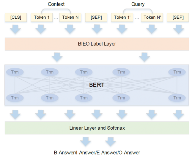
Figure 3. The structure of the BERT model proposed in this study. [CLS] and [SEP] are special markers that identify the beginning and end of an input text. [CLS] stands for “classification”, and adding a [CLS] token at the beginning of the input text allows the model to learn a representation for the whole sentence. [SEP] stands for “separator”, used mainly to separate different sentences or pieces of text. The “Trm” inside BERT represents the transformer architecture.
