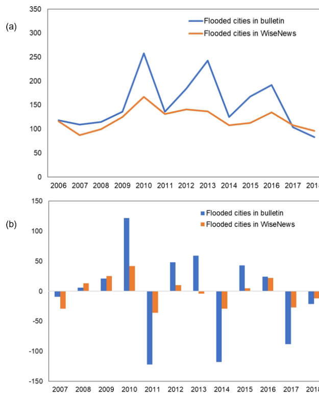
Figure 4. The comparison between the number of flooded cities extracted from the news and the China Flood and Drought Bulletin for each year. (a) The time series of both datasets. (b) Year-to-year changes in both datasets, with the y axis showing the difference in values from the previous year. The positive bars indicate an increase compared to the previous year, whereas the negative bars indicate a decrease.
