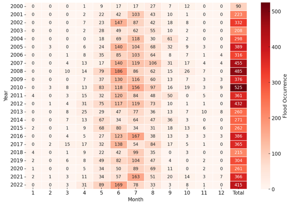
Figure 5. A heatmap showing in each cell the number of flood occurrences for each month and each year.
