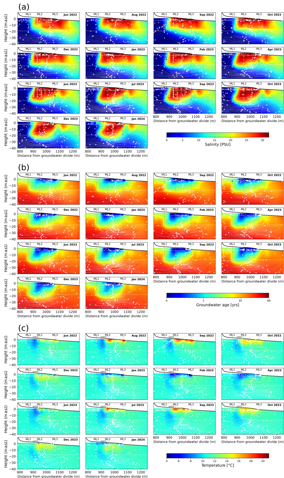
Figure 4. Simulated (heat map) and observed (circles) data of (a) salinity, (b) groundwater age and (c) temperature. Dates in the top-right corner show the sampling dates and the corresponding model simulation times. The white arrows represent the groundwater flow directions, and the arrow thickness indicates the pore-water velocity.
