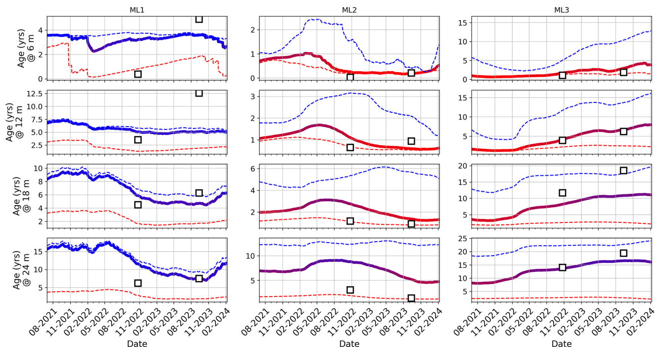
Figure 5. Simulated ages of seawater component (dashed red), freshwater component (dashed blue) and groundwater direct age (solid, varying from blue to red depending on salinity), and observed ^3\text{H}/^4\text{He} groundwater age (squares). The ages of the sea- and freshwater components were calculated from saltwater-freshwater endmember mixing and the computed direct groundwater age.
