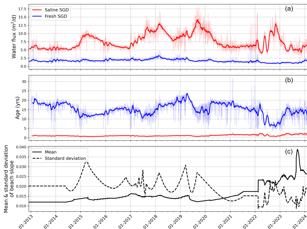
Figure 7. (a) Simulated time series of saline (red) and fresh (blue) SGD water flux. Thin lines represent the fluxes derived half-daily after each stress period, thick lines represent the signal smoothed with a Savitzky-Golay filter with a polynomial order of 2 and a window length encompassing 101 data points. (b) Simulated time series of flux weighted groundwater ages of the saline (red) and fresh (blue) SGD components. Thin lines represent the fluxes derived half-daily after each stress period, thick lines represent the signal smoothed with a Savitzky-Golay filter with a polynomial order of 2 and a window length encompassing 101 data points. (c) Mean and standard deviation of the beach slope in the intertidal zone. Only the time-period from January 2013 onwards are presented, i.e., the period where the dynamics of the sea side boundary condition is considered in the model.
