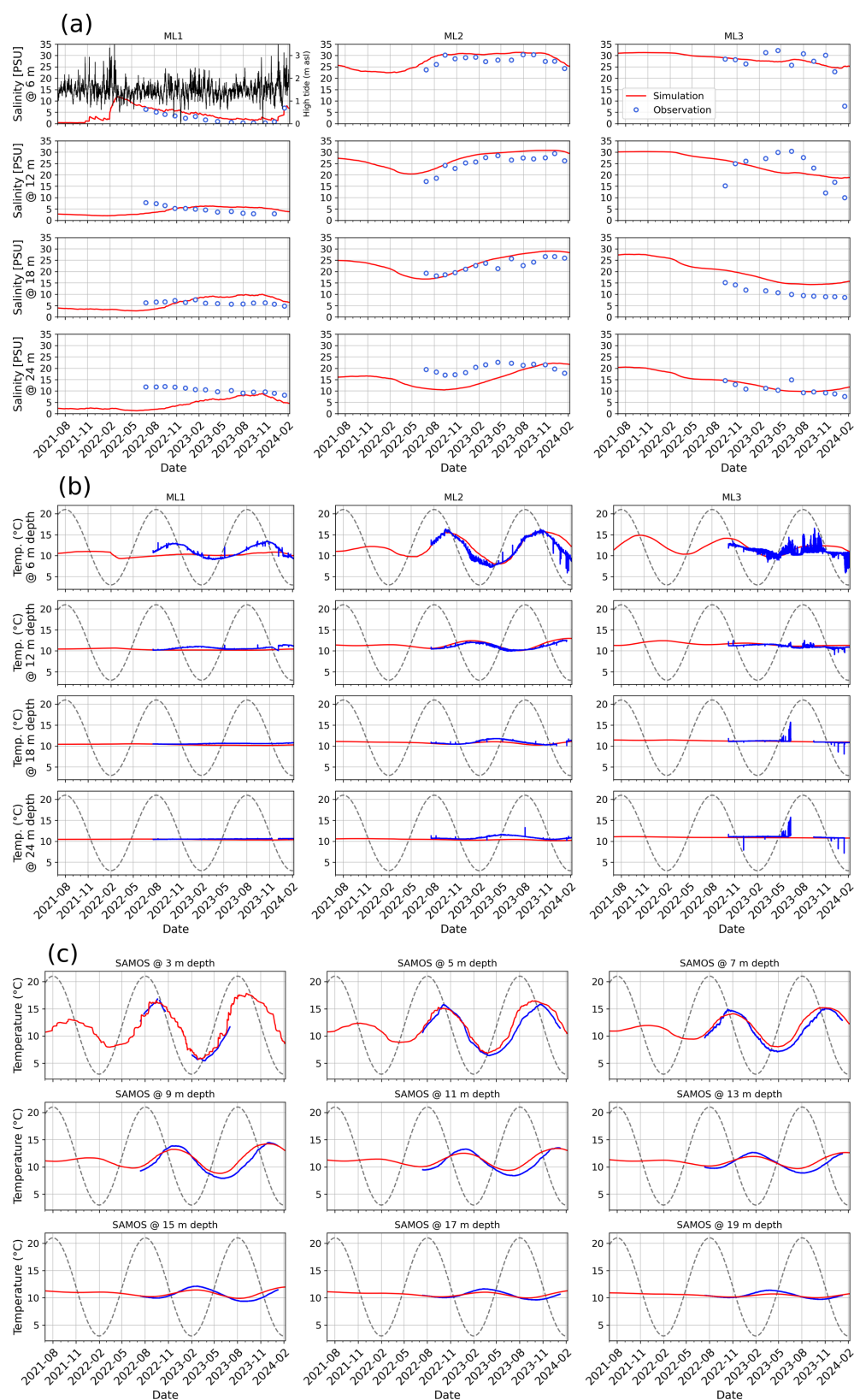
Figure 3. (a) Simulated (red line) and observed data of salinity (blue circles) and (b) temperature (blue line) at multi-level observation wells and (c) temperature (blue line) SAMOS. In panel (a), the black line represents the sea level at high tide and is the sum of high tide and wave setup. In plot B and C, the grey dashed line represents the sea water temperature.
