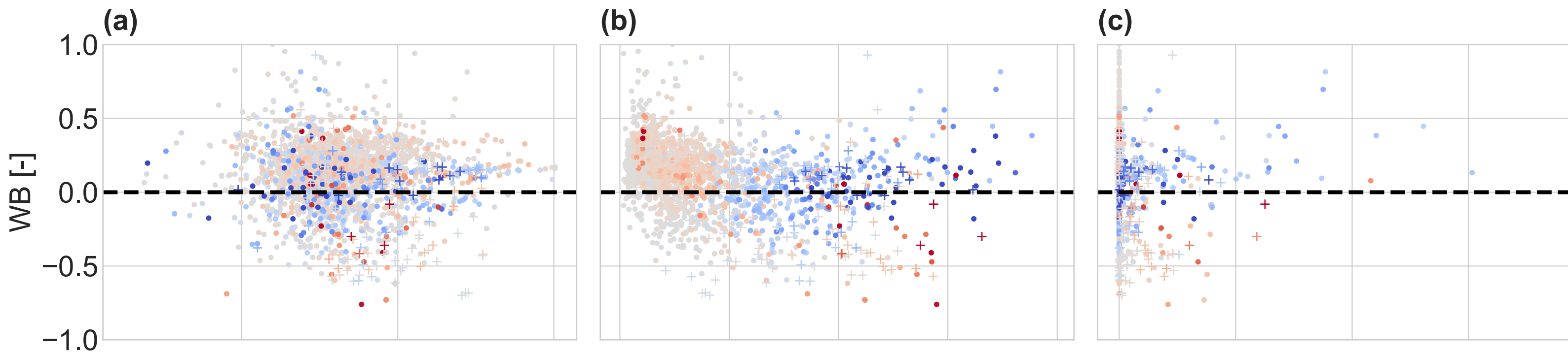
Glaciers (Snow and glaciers vs Calibrated snow)
