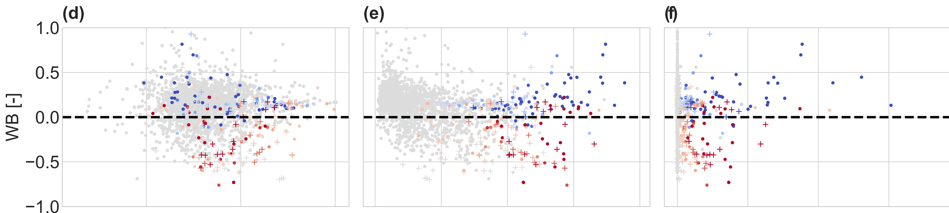
Soil (Full model vs Snow and glaciers)
