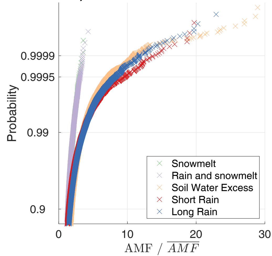
b) Floods - RCP4.5 2070-2100
