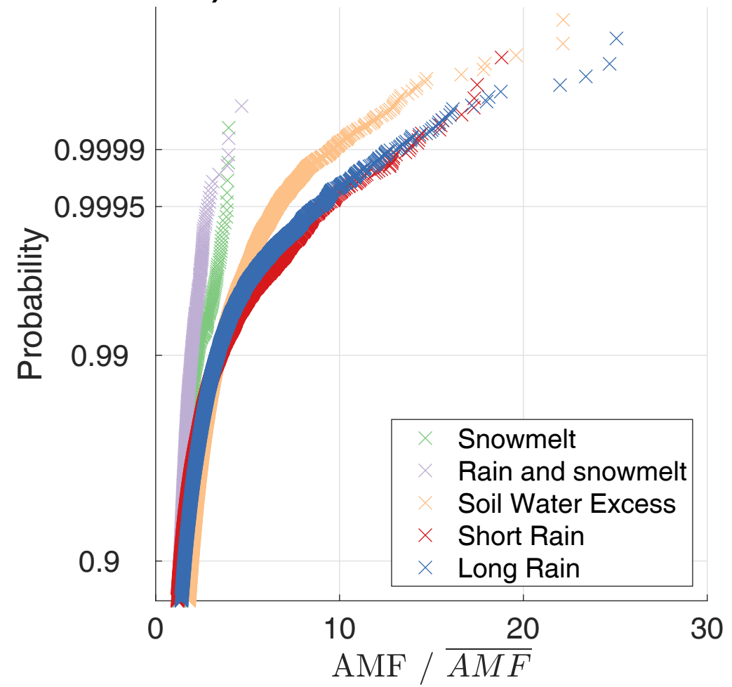
c) Floods - RCP8.5 2070-2100
