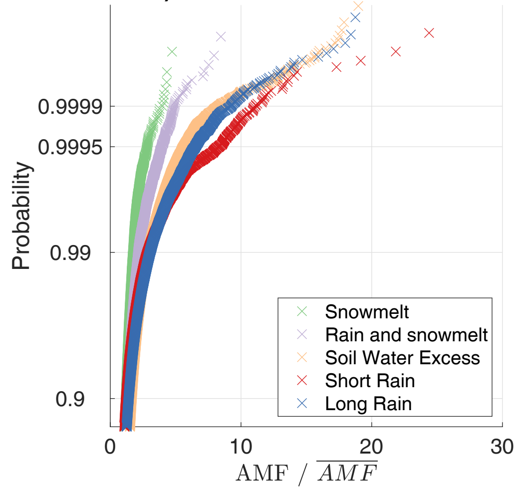
a) Floods - HIST 1975-2005
