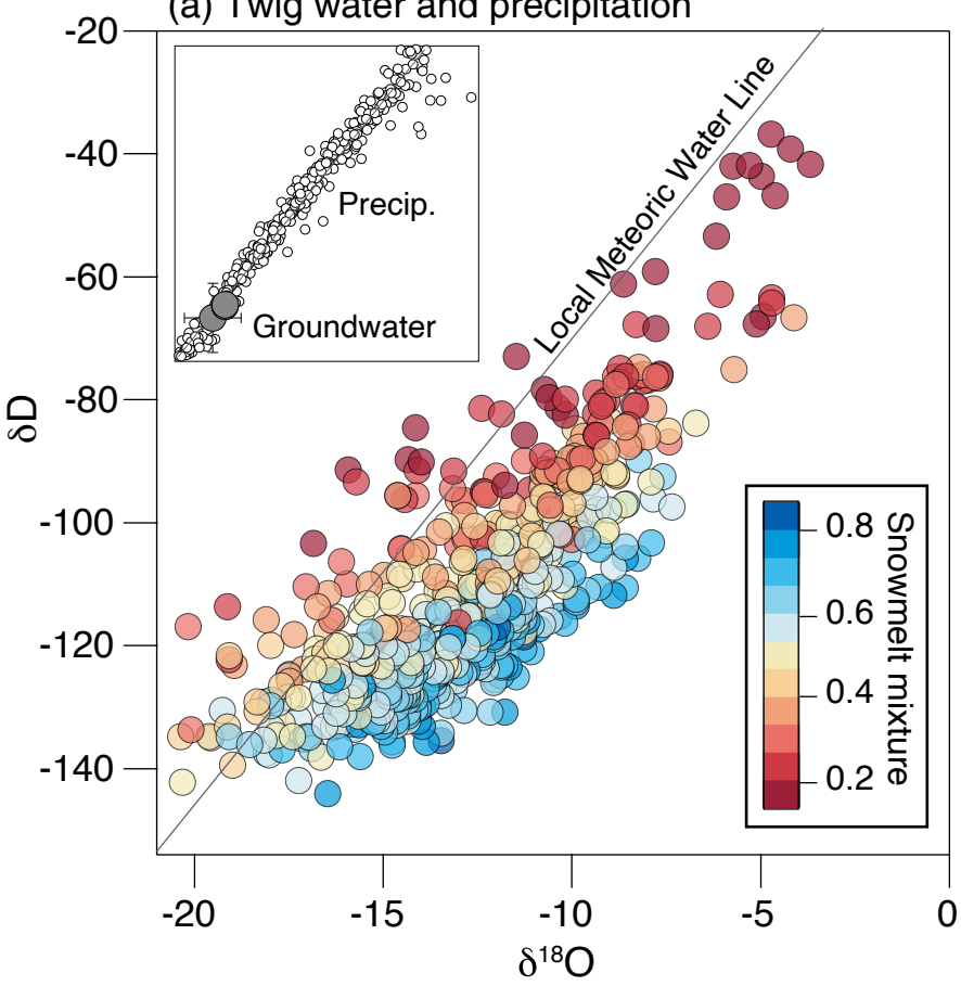
(a) Twig water and precipitation
