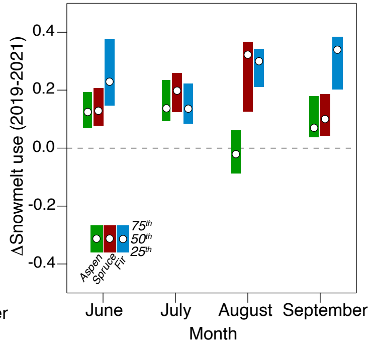
(c) \Delta Snowmelt use by month & species
