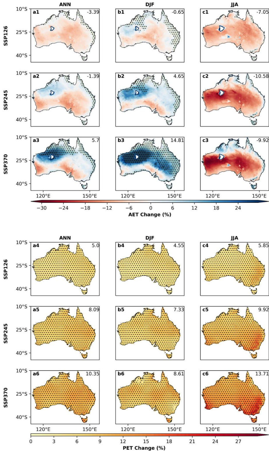
Figure S1: Bias corrected climate change patterns for AET and PET across annual (ANN), summer (DJF), winter (JJA) seasons in Australia. Projected climate change patterns are shown for 2080-2099 with respect to 1995-2014. Results are shown for 11-model ensemble mean under emissions scenarios (SSP126, SSP245 and SSP370). Bias correction used AWO datasets as reference. Stippling shown where the signal-to-noise ratio > 1.
