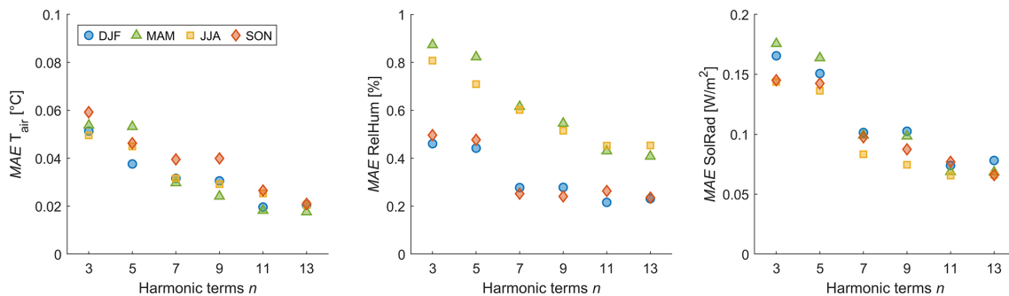
Figure 3. Seasonal mean absolute error (MAE) between historical timeseries and timeseries smoothed with n harmonic terms for air temperature (left), relative humidity (middle) and solar radiation (right).
