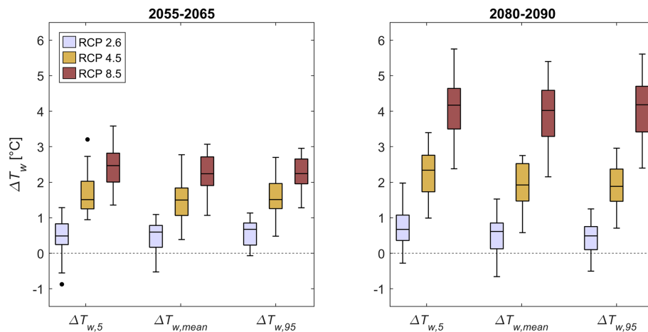
Figure 8. Simulated difference between current (2019–2021) and future climate for the mean annual temperature ( \Delta T_{w,mean} ), the 5th and 95th percentiles of annual temperature ( \Delta T_{w,5} and \Delta T_{w,95} ). Temperatures are averaged on the entire river reach.
