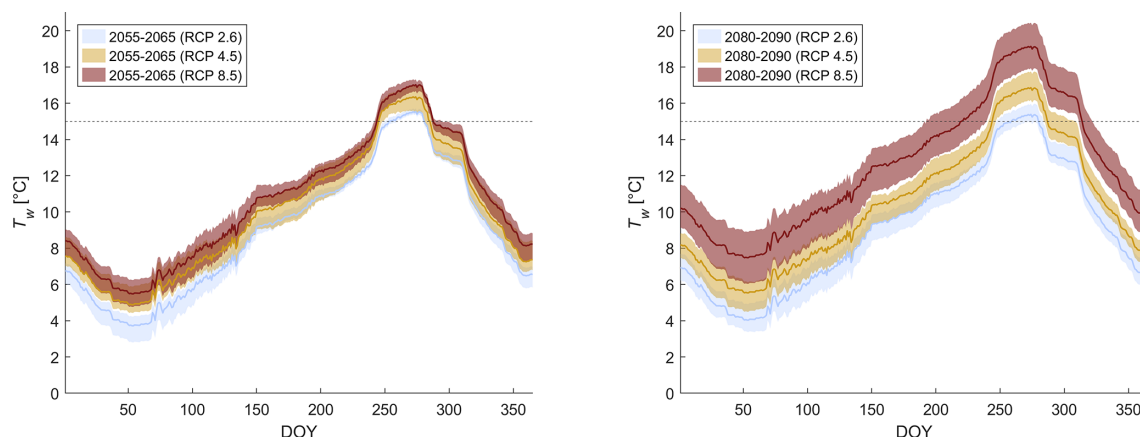
Figure B3. Simulated lake temperature at residual for intake level (637.5 m a.s.l.) under climate change for 2055–2065 (left) and 2080–2090 (right), dotted line indicates 15 °C showing that lake temperature will tend to be above this threshold more often in the future.
