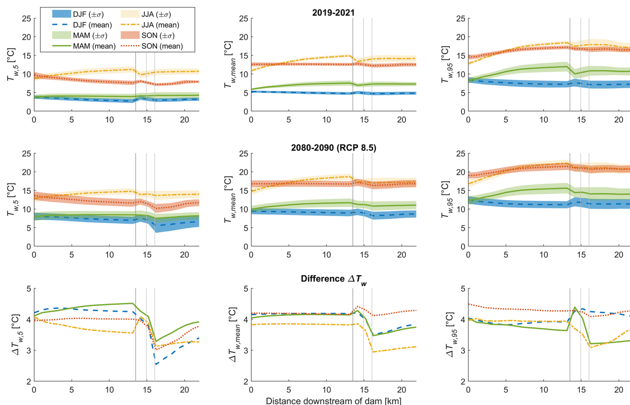
Figure C1. Simulated seasonal temperature along the reach under current climate (top, 2019–2021) and future climate (middle, for 2080–2090 and RC P8.5) with the 5th percentile, the mean and the 95th percentile of the seasonal values, and difference between these simulated temperature indicators under future and current climate (bottom).
