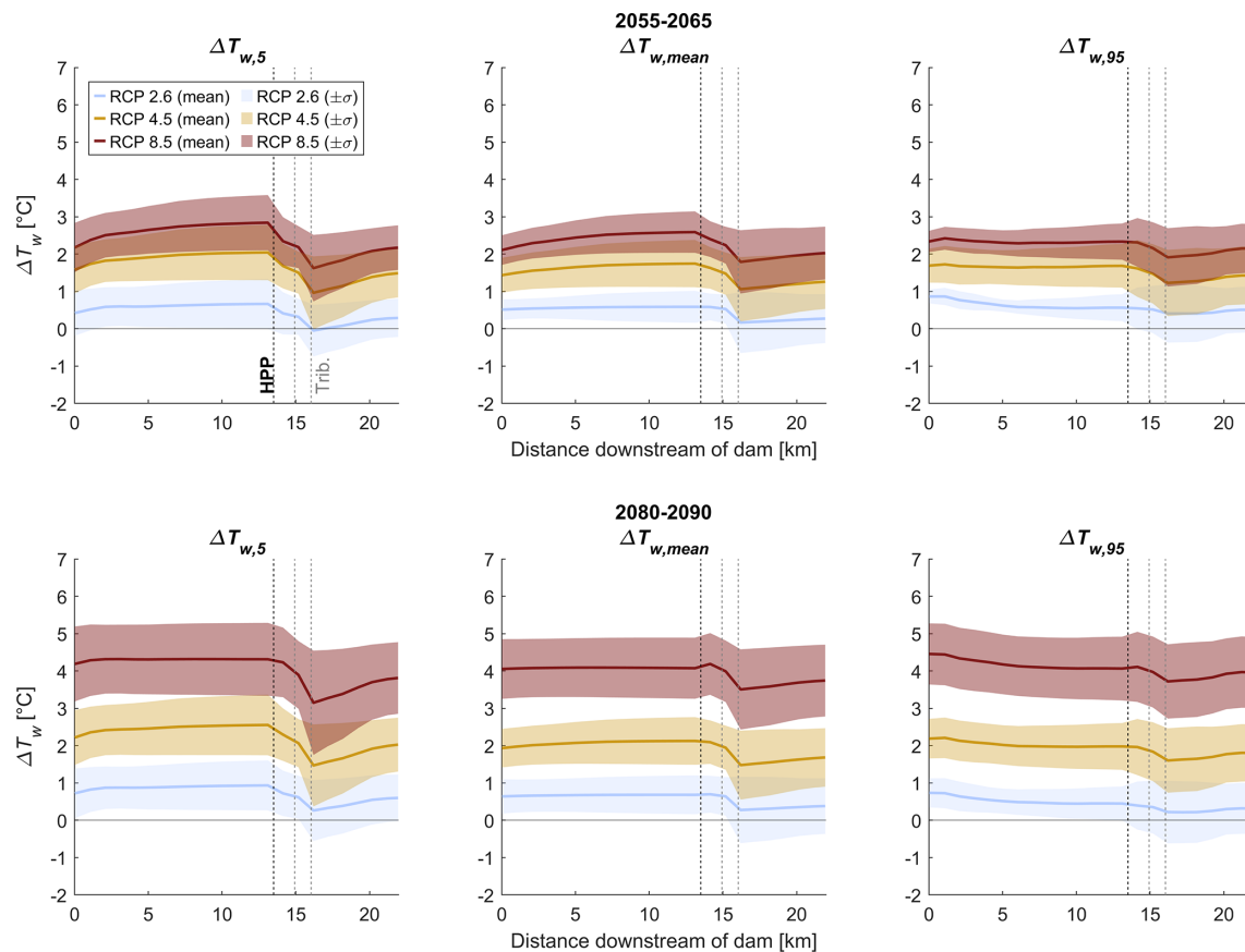
Figure 10. Spatial distribution of simulated difference between current (2019–2021) and future climate for the mean annual temperature ( \Delta T_{w,\text{mean}} ), the 5th and 95th percentiles of annual temperature ( \Delta T_{w,5} and \Delta T_{w,95} ). The black line (HPP) shows the section where water is released from hydropower plant and the two grey lines (Trib.) show the confluence sections with the two tributaries.
