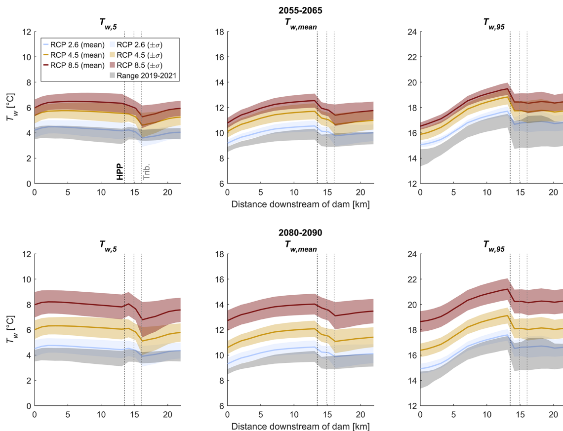
Figure 9. Simulated stream temperature along the investigated river reach for the current climate (2019–2021) and future climate (top: 2055–2065; bottom: 2080–2090) for the mean annual temperature ( T_{w,mean} ), the 5th and 95th percentiles of annual temperature ( T_{w,5} and T_{w,95} ). The black line (HPP) shows the section where water is released from hydropower plant and the two grey lines (Trib.) show the confluence sections with the two tributaries.
