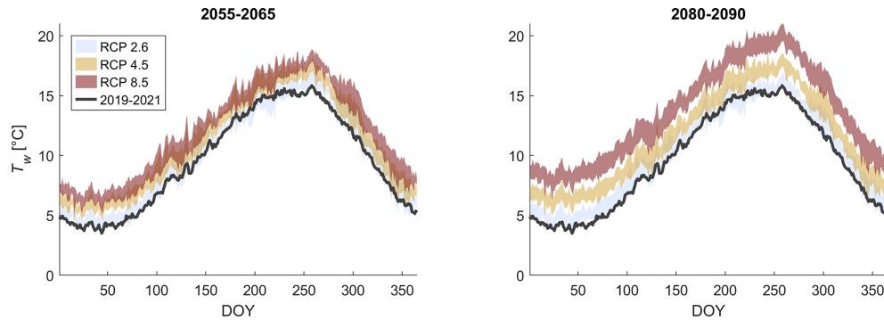
Figure 7. Simulated temperatures for the current climate (average from 2019 to 2021) and future projections. The shaded areas indicate the range of variability across different simulations for the same RCP scenario. Temperatures are averaged on the entire river reach.
