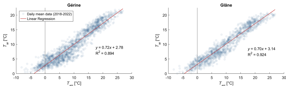
Figure 6. Correlation between daily mean air temperature and daily mean stream temperature for both tributaries (G rine, left and Gl ne, right).
