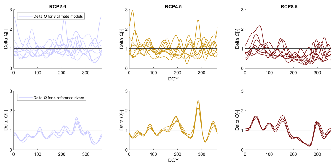
Figure 4. Variability of the smoothed discharge-delta computed based on different climate models but on the same reference river (top) and based on 4 different reference rivers but with the same climate model (bottom, with climate model No. 2 from Table 1).
