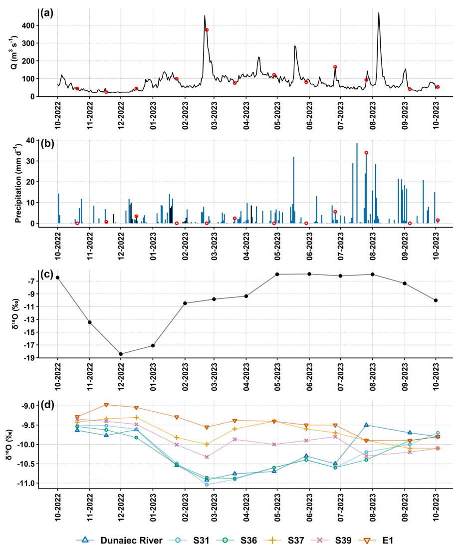
Figure 4. Mean daily flow rates of the Dunajec River at the Zgłobice water-gauging station (a), daily precipitation in Tarnów in the form of rain (blue) or snow (black) (b), monthly means of \delta^{18}\text{O} in precipitation (Kraków station) (c), as well as \delta^{18}\text{O} in the Dunajec River water and groundwater in the study area throughout the sampling period (October 2022–October 2023). Red circles on plots (a) and (b) indicate the days of water sampling.
