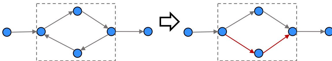
Constraint 7: no recirculation inside the cycles
