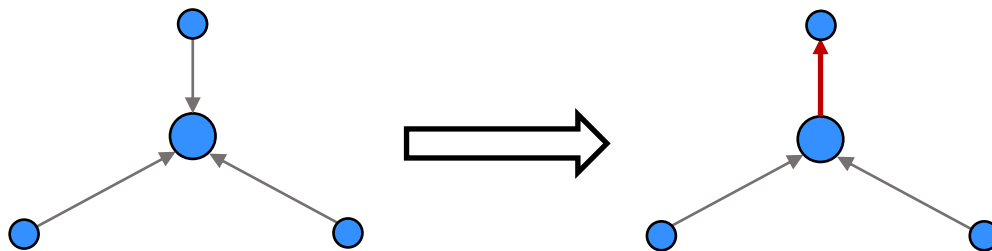
Constraint 5: strictly positive out-degrees at non-outfall nodes
