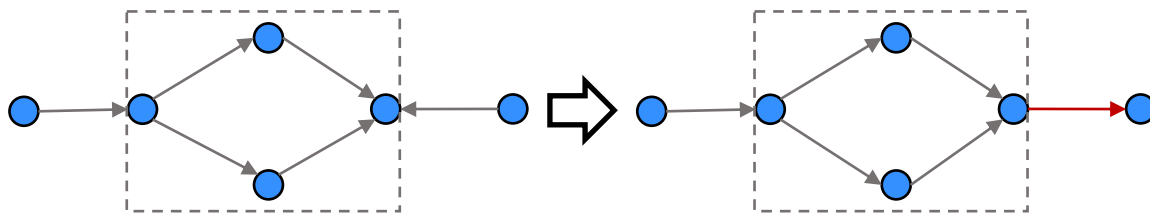
Constraint 6: strictly positive out-degrees of cycles
