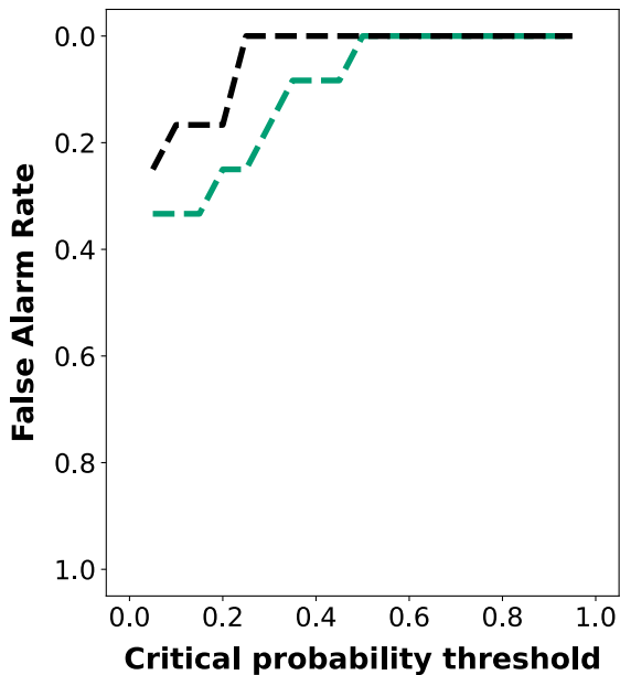
(b) USGS 09124500 - Lake Fork, CO
