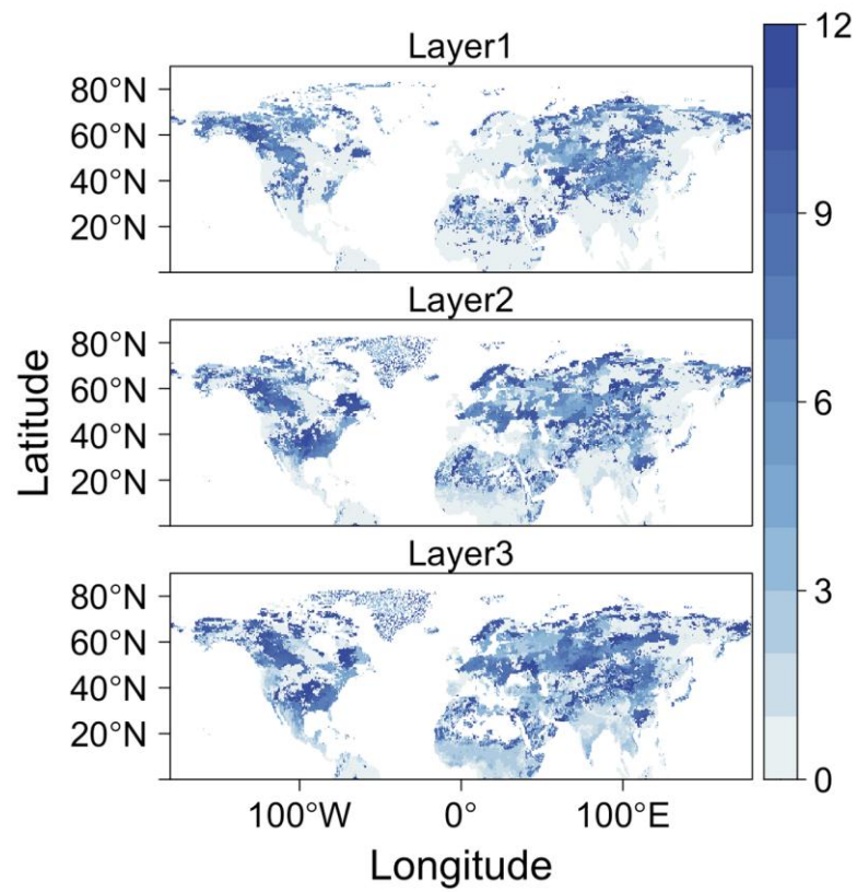
Fig. S2 The estimated number of lagged month for each grid in the the Kendall's tau correlation.
