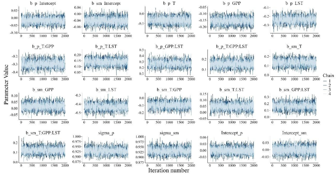
Fig. S4 Markov Chain trace plots for annual model parameter sampling.
