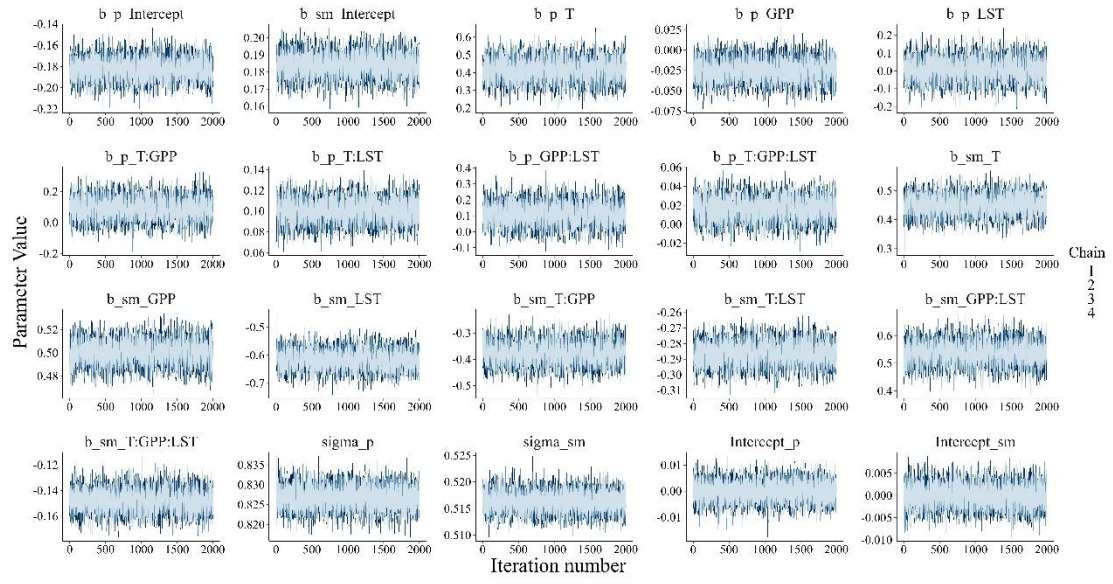
Fig. S3 Markov Chain trace plots for monthly model parameter sampling.
