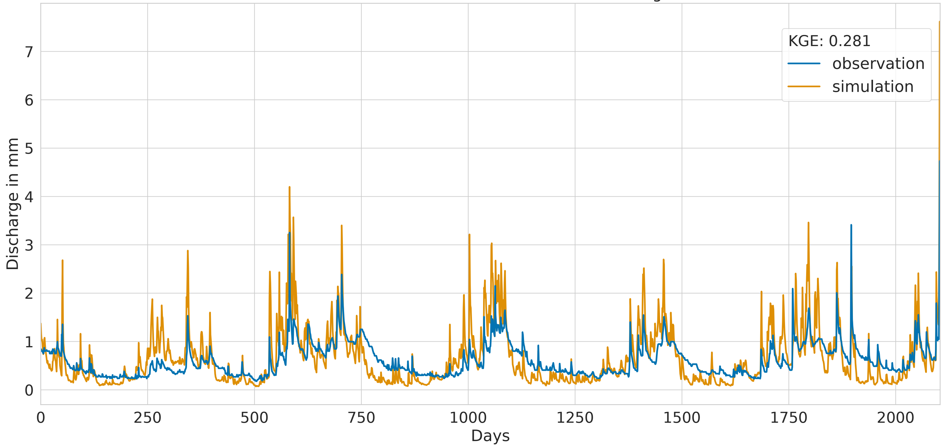
GRU with static features and batch size of 256 for Gauge 41860900
