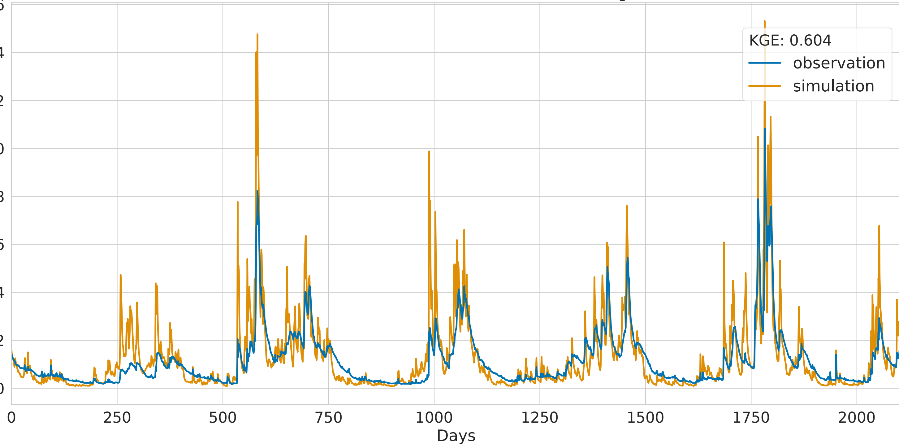
GRU with static features and batch size of 256 for Gauge 24480695
