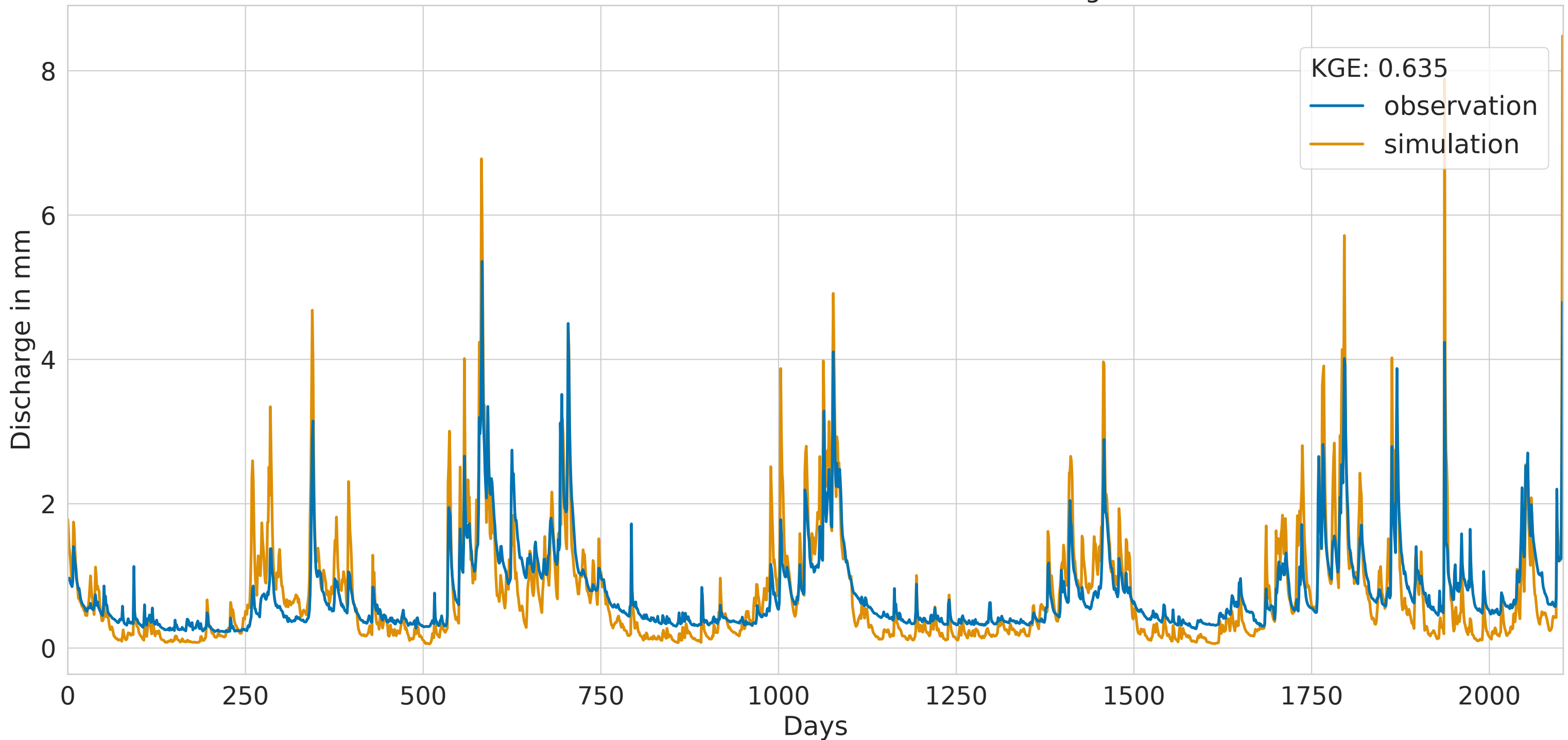
GRU with static features and batch size of 256 for Gauge 44950055
