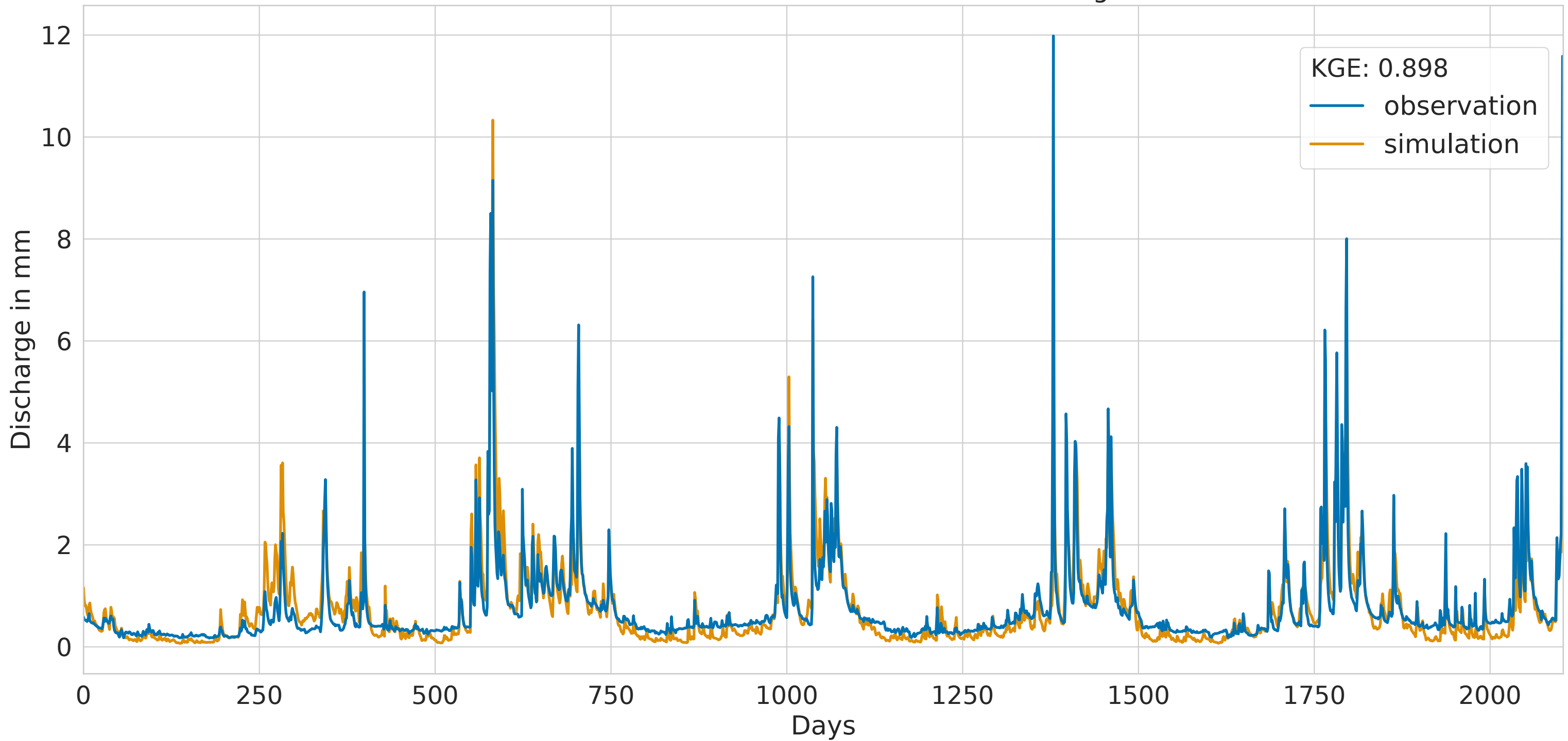
GRU with static features and batch size of 256 for Gauge 25811255
