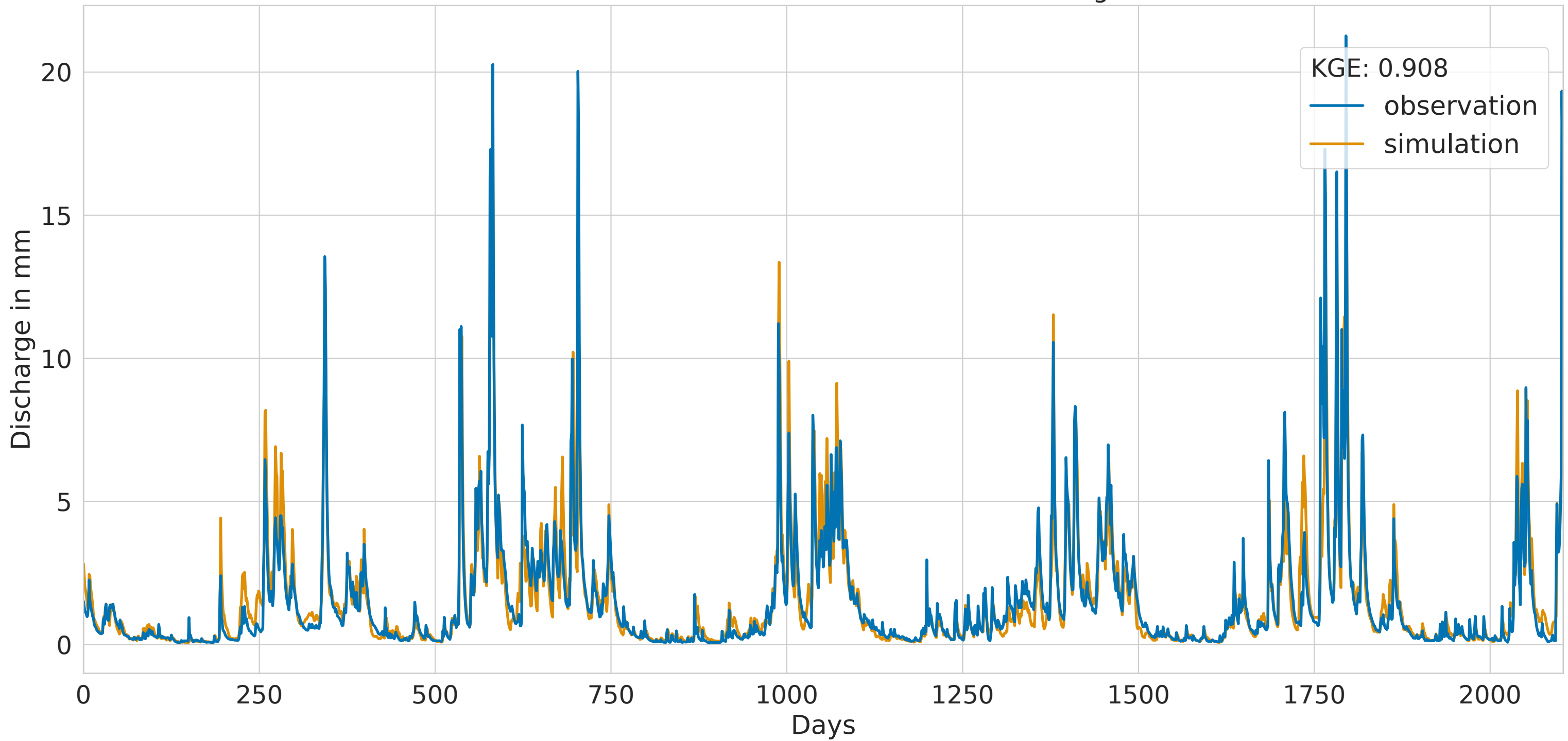
GRU with static features and batch size of 256 for Gauge 25840708
