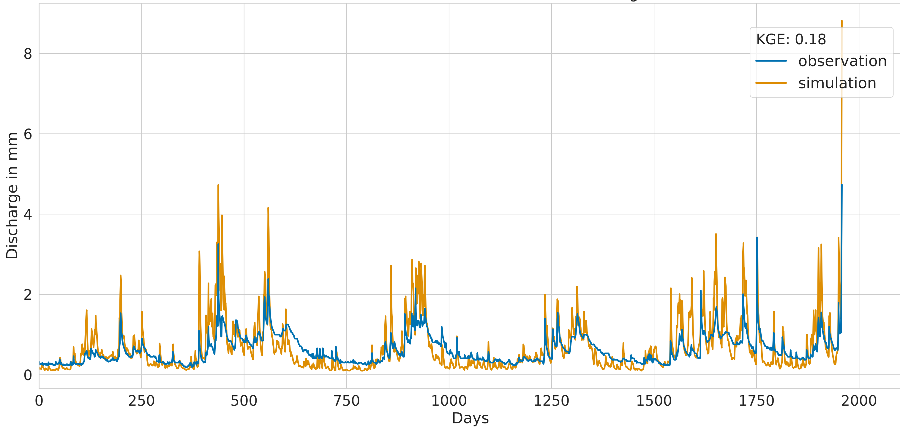
LSTM with static features and batch size of 256 for Gauge 41860900
