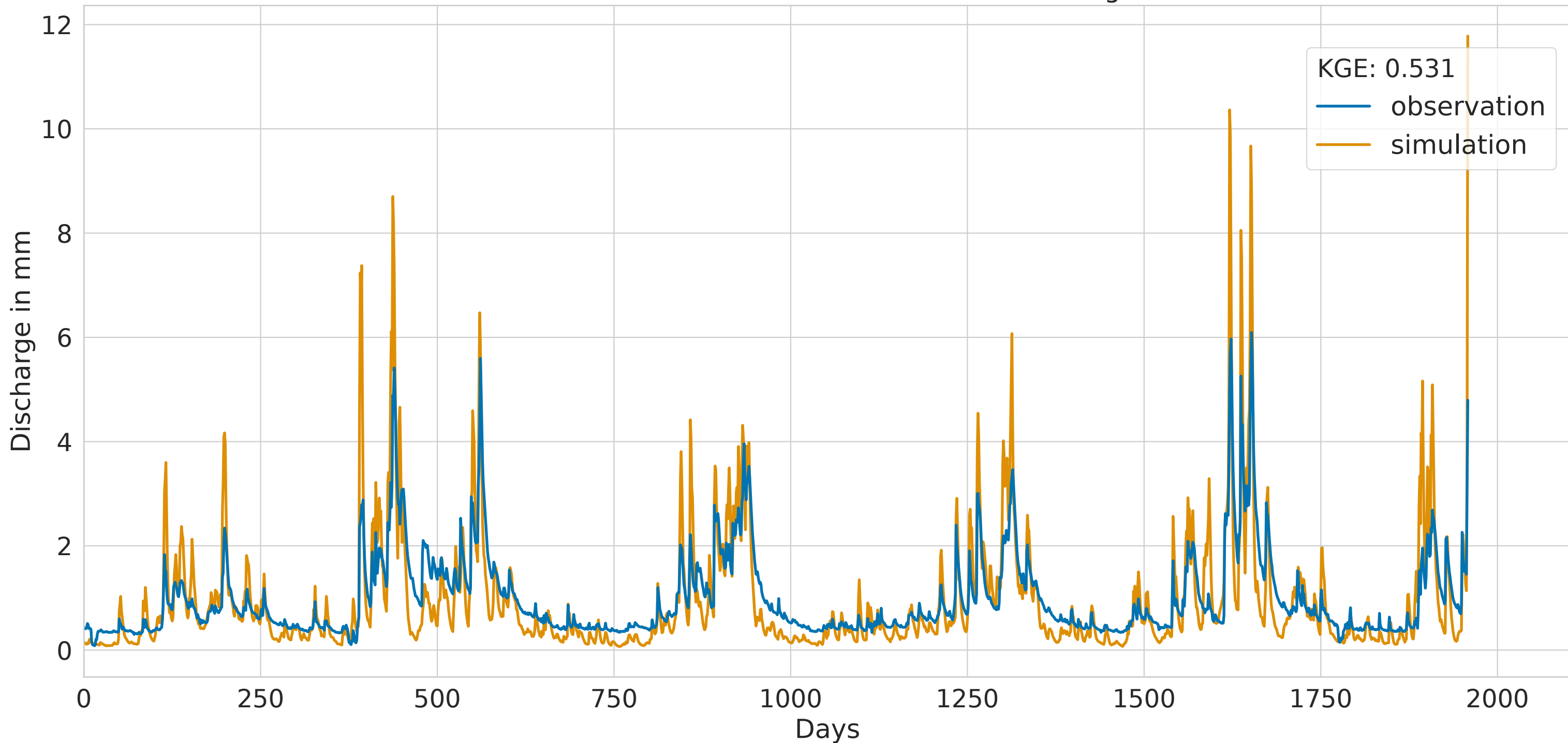
LSTM with static features and batch size of 256 for Gauge 41510205
