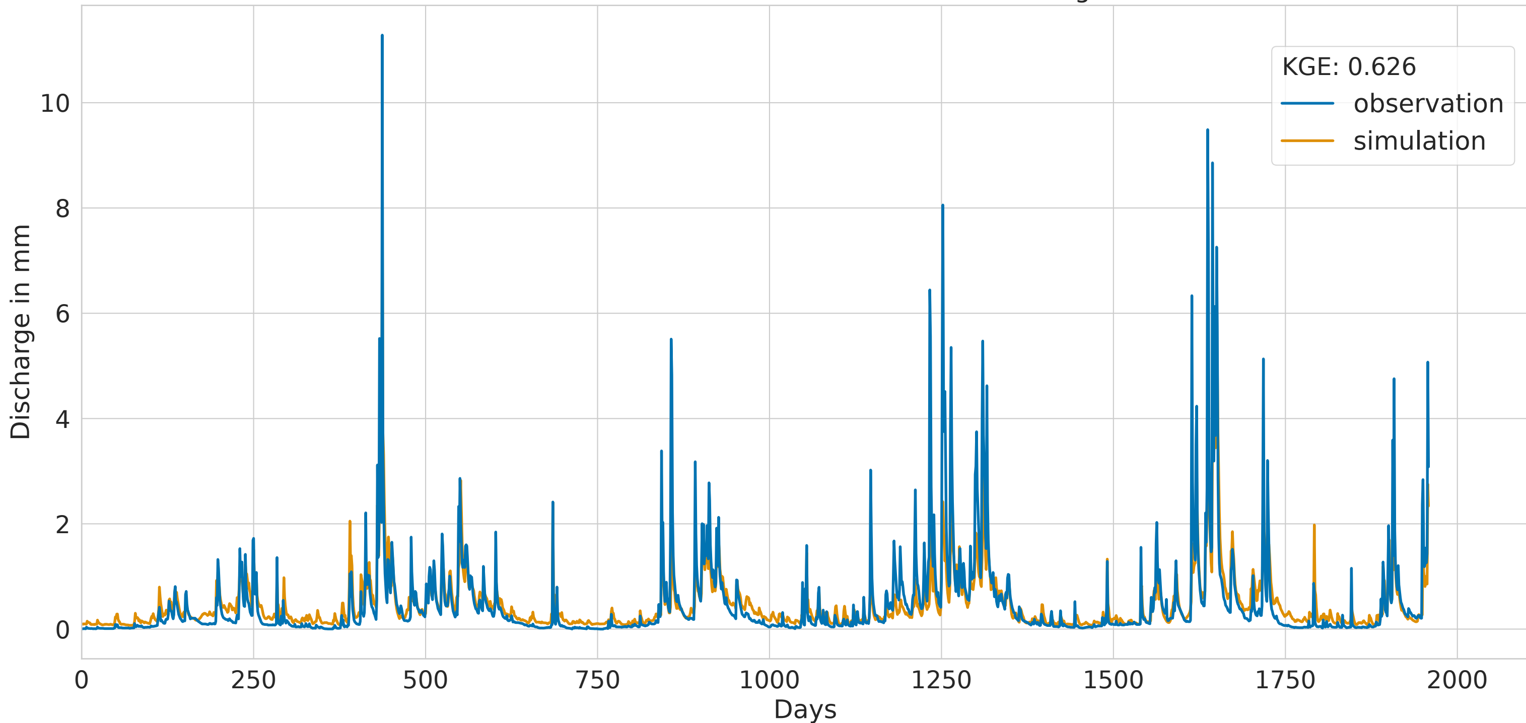
LSTM with static features and batch size of 256 for Gauge 24880208
