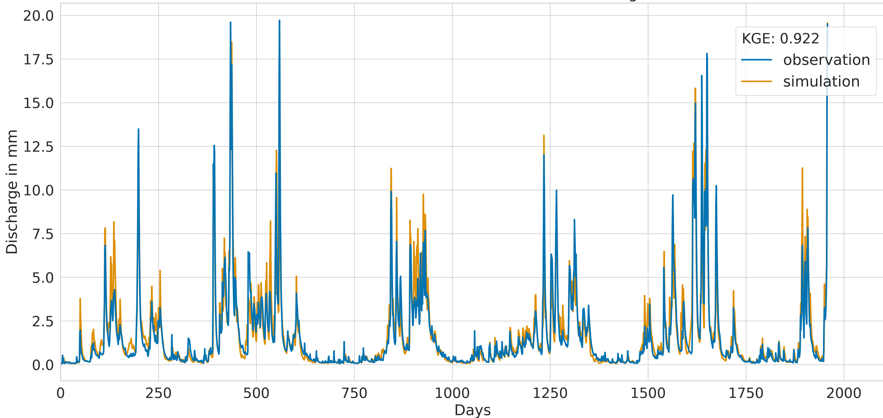
LSTM with static features and batch size of 256 for Gauge 25840650
