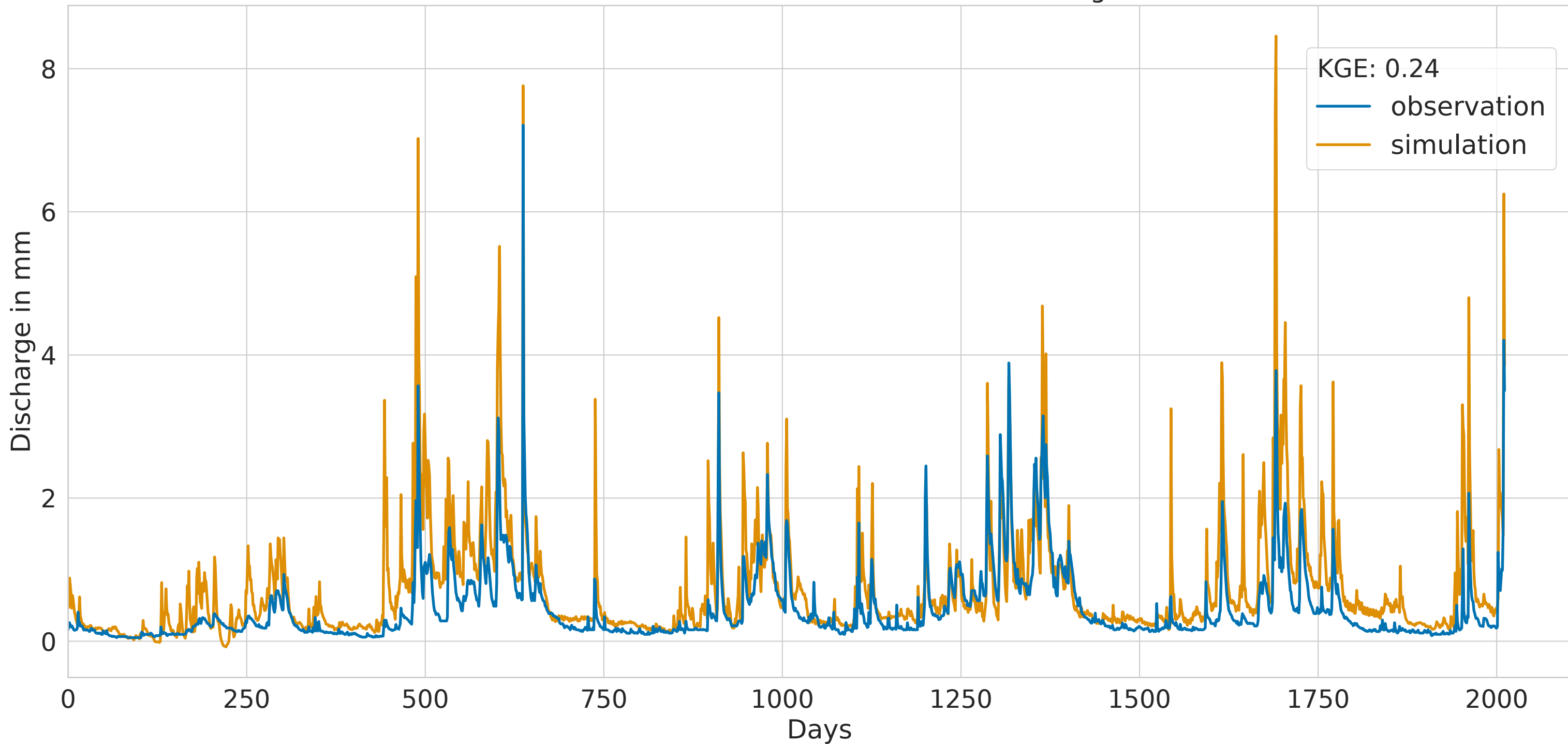
CNN with static features and batch size of 256 for Gauge 25140058
